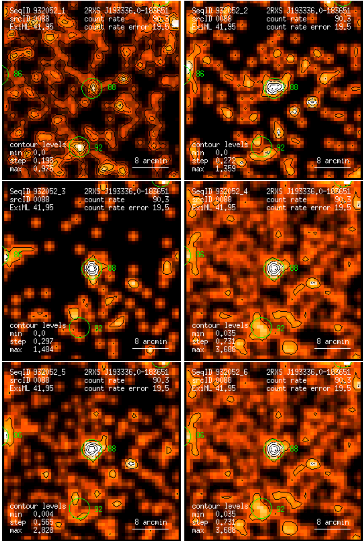
Figure 88: RASS 932052: detection 0088: band rate images, Gaussian filter: (1) PSPC channels 11 – 41, (2) 52 – 90, (3) 91 – 201, (4) 11 – 235, (5) 52 – 201, (6) 11 – 201. Broad band rates in counts/ks. Band rate contour levels in counts/ks/arcmin 2 .
