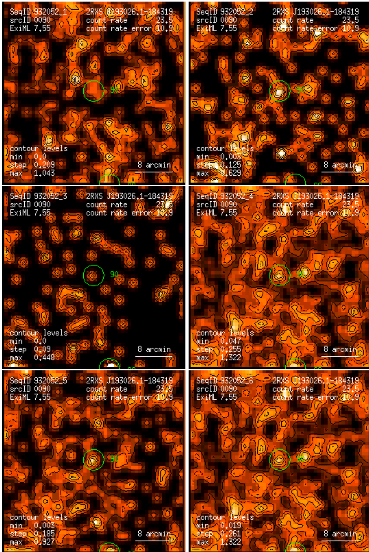
Figure 90: RASS 932052: detection 0090: band rate images, Gaussian filter: (1) PSPC channels 11 – 41, (2) 52 – 90, (3) 91 – 201, (4) 11 – 235, (5) 52 – 201, (6) 11 – 201. Broad band rates in counts/ks. Band rate contour levels in counts/ks/arcmin 2 .
