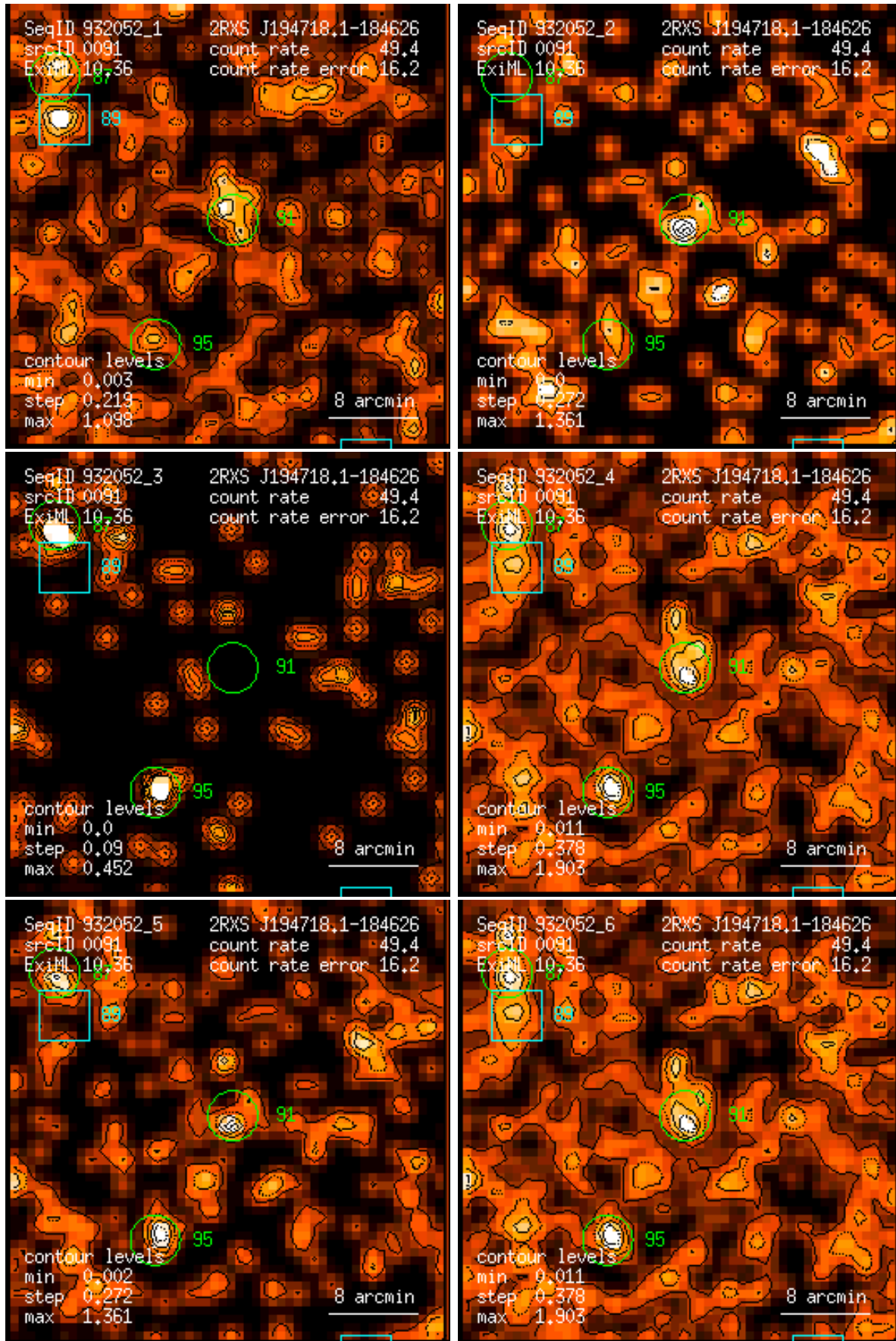
Figure 91: RASS 932052: detection 0091: band rate images, Gaussian filter: (1) PSPC channels 11 – 41, (2) 52 – 90, (3) 91 – 201, (4) 11 – 235, (5) 52 – 201, (6) 11 – 201. Broad band rates in counts/ks. Band rate contour levels in counts/ks/arcmin 2 .
