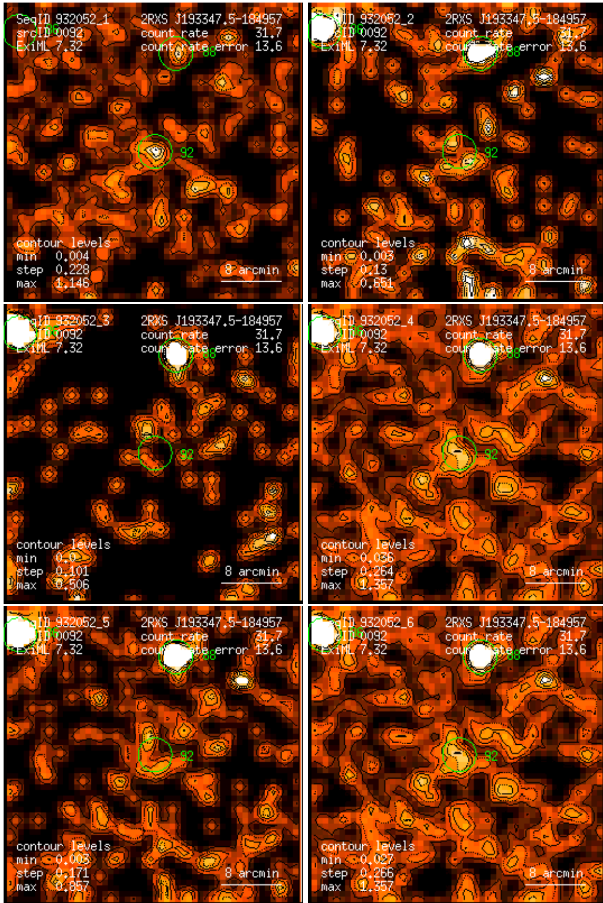
Figure 92: RASS 932052: detection 0092: band rate images, Gaussian filter: (1) PSPC channels 11 – 41, (2) 52 – 90, (3) 91 – 201, (4) 11 – 235, (5) 52 – 201, (6) 11 – 201. Broad band rates in counts/ks. Band rate contour levels in counts/ks/arcmin 2 .
