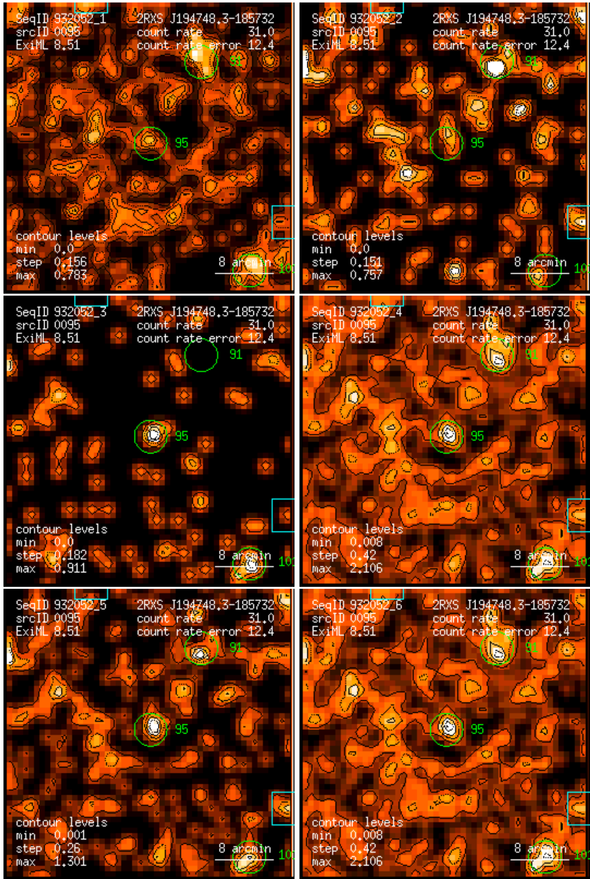
Figure 95: RASS 932052: detection 0095: band rate images, Gaussian filter: (1) PSPC channels 11 – 41, (2) 52 – 90, (3) 91 – 201, (4) 11 – 235, (5) 52 – 201, (6) 11 – 201. Broad band rates in counts/ks. Band rate contour levels in counts/ks/arcmin 2 .
