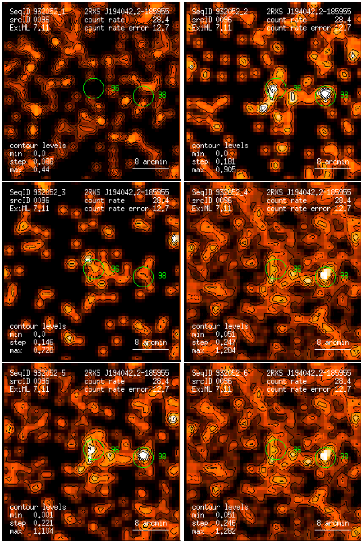
Figure 96: RASS 932052: detection 0096: band rate images, Gaussian filter: (1) PSPC channels 11 – 41, (2) 52 – 90, (3) 91 – 201, (4) 11 – 235, (5) 52 – 201, (6) 11 – 201. Broad band rates in counts/ks. Band rate contour levels in counts/ks/arcmin 2 .
