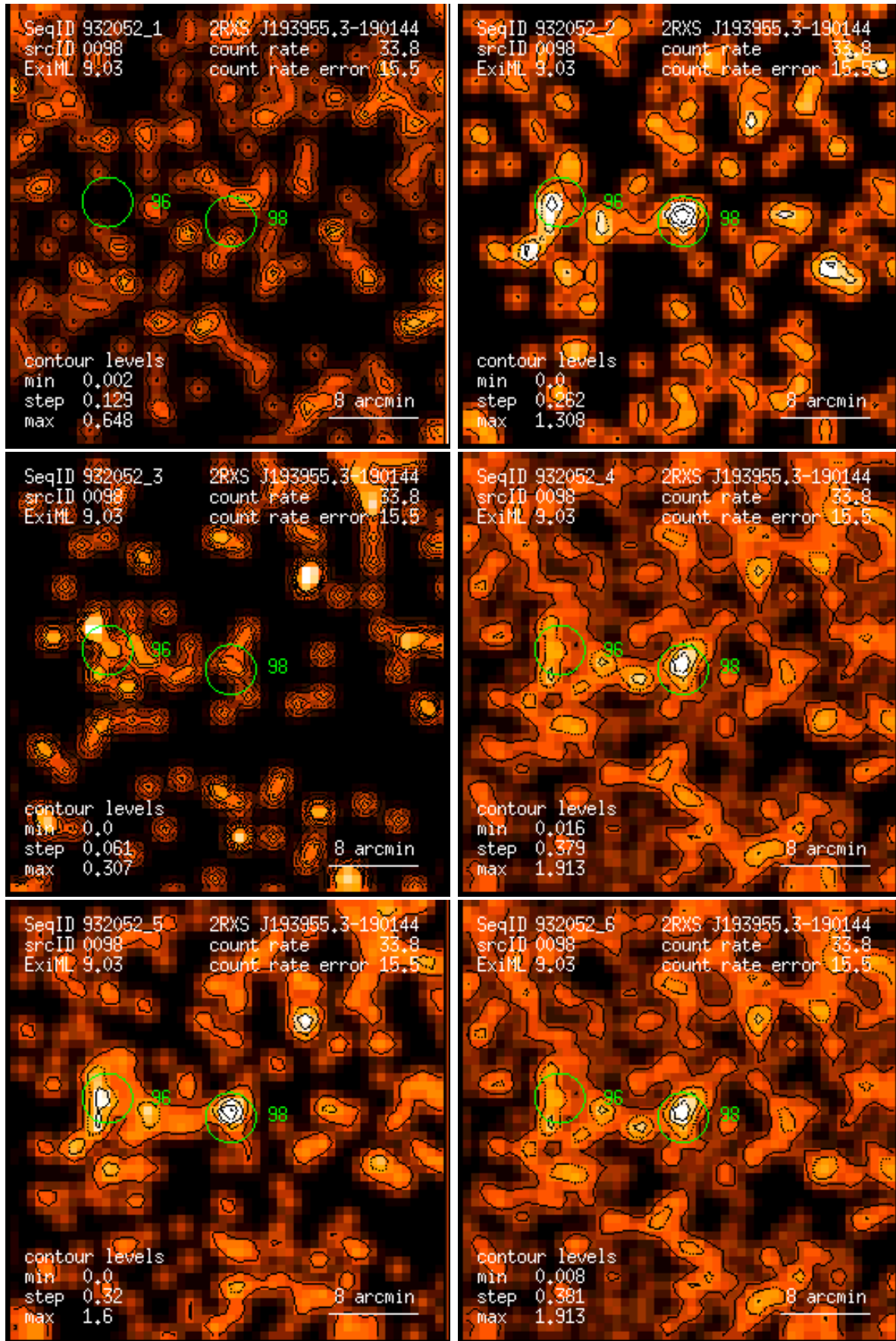
Figure 98: RASS 932052: detection 0098: band rate images, Gaussian filter: (1) PSPC channels 11 – 41, (2) 52 – 90, (3) 91 – 201, (4) 11 – 235, (5) 52 – 201, (6) 11 – 201. Broad band rates in counts/ks. Band rate contour levels in counts/ks/arcmin 2 .
