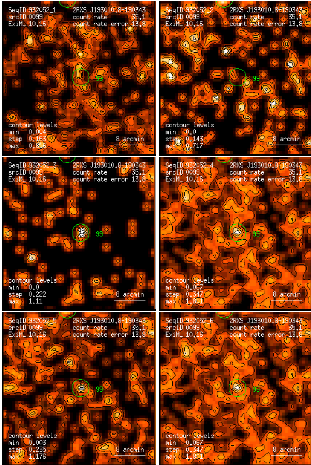
Figure 99: RASS 932052: detection 0099: band rate images, Gaussian filter: (1) PSPC channels 11 – 41, (2) 52 – 90, (3) 91 – 201, (4) 11 – 235, (5) 52 – 201, (6) 11 – 201. Broad band rates in counts/ks. Band rate contour levels in counts/ks/arcmin 2 .
