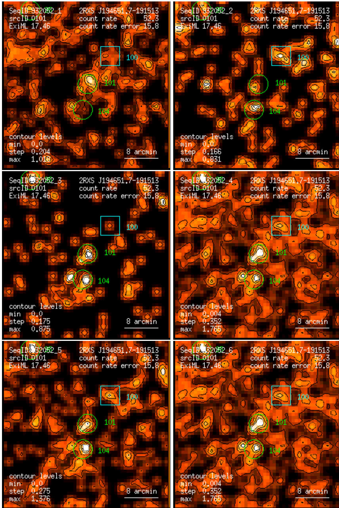
Figure 101: RASS 932052: detection 0101: band rate images, Gaussian filter: (1) PSPC channels 11 – 41, (2) 52 – 90, (3) 91 – 201, (4) 11 – 235, (5) 52 – 201, (6) 11 – 201. Broad band rates in counts/ks. Band rate contour levels in counts/ks/arcmin 2 .
