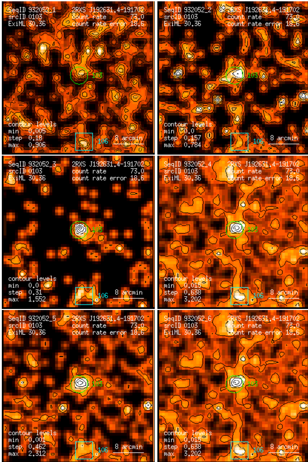
Figure 103: RASS 932052: detection 0103: band rate images, Gaussian filter: (1) PSPC channels 11 – 41, (2) 52 – 90, (3) 91 – 201, (4) 11 – 235, (5) 52 – 201, (6) 11 – 201. Broad band rates in counts/ks. Band rate contour levels in counts/ks/arcmin 2 .
