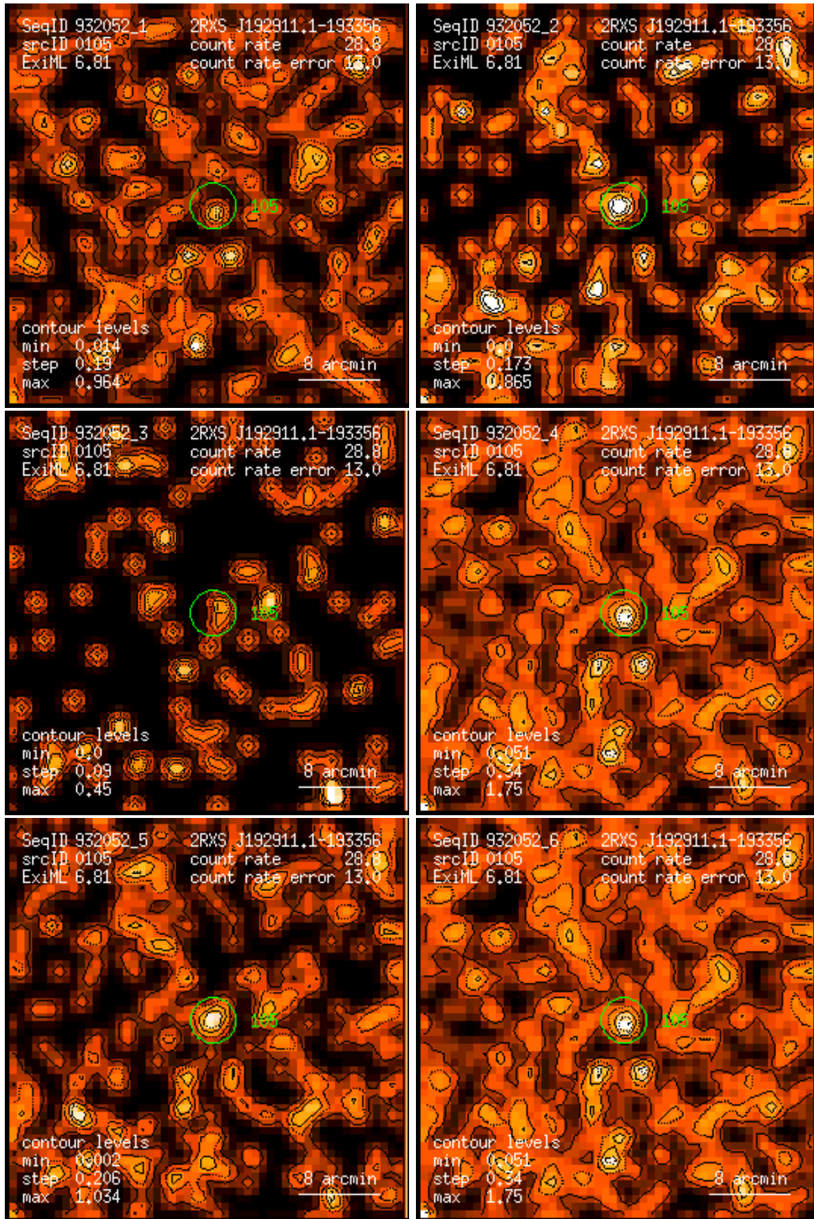
Figure 105: RASS 932052: detection 0105: band rate images, Gaussian filter: (1) PSPC channels 11 – 41, (2) 52 – 90, (3) 91 – 201, (4) 11 – 235, (5) 52 – 201, (6) 11 – 201. Broad band rates in counts/ks. Band rate contour levels in counts/ks/arcmin 2 .
