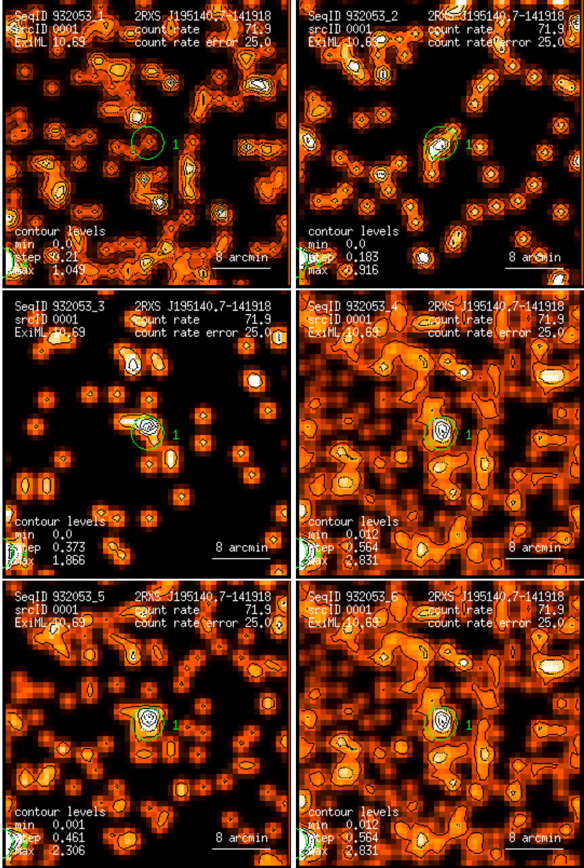
Figure 1: RASS 932053: detection 0001: band rate images, Gaussian filter: (1) PSPC channels 11 – 41, (2) 52 – 90, (3) 91 – 201, (4) 11 – 235, (5) 52 – 201, (6) 11 – 201. Broad band rates in counts/ks. Band rate contour levels in counts/ks/arcmin 2 .
