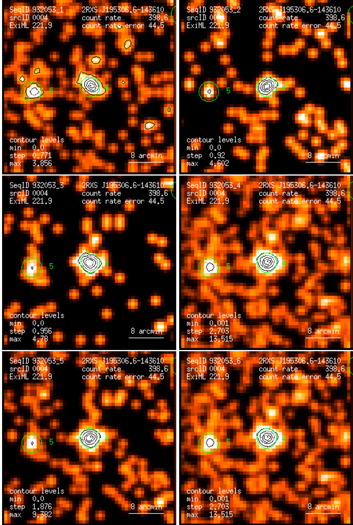
Figure 4: RASS 932053: detection 0004: band rate images, Gaussian filter: (1) PSPC channels 11 – 41, (2) 52 – 90, (3) 91 – 201, (4) 11 – 235, (5) 52 – 201, (6) 11 – 201. Broad band rates in counts/ks. Band rate contour levels in counts/ks/arcmin 2 .
