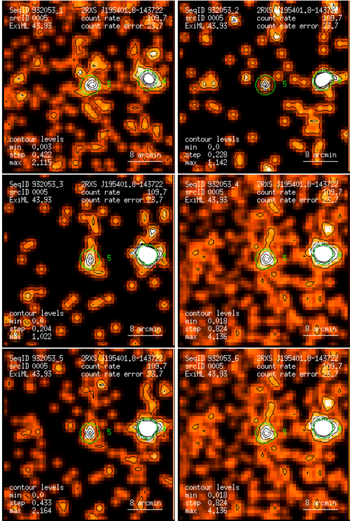
Figure 5: RASS 932053: detection 0005: band rate images, Gaussian filter: (1) PSPC channels 11 – 41, (2) 52 – 90, (3) 91 – 201, (4) 11 – 235, (5) 52 – 201, (6) 11 – 201. Broad band rates in counts/ks. Band rate contour levels in counts/ks/arcmin 2 .
