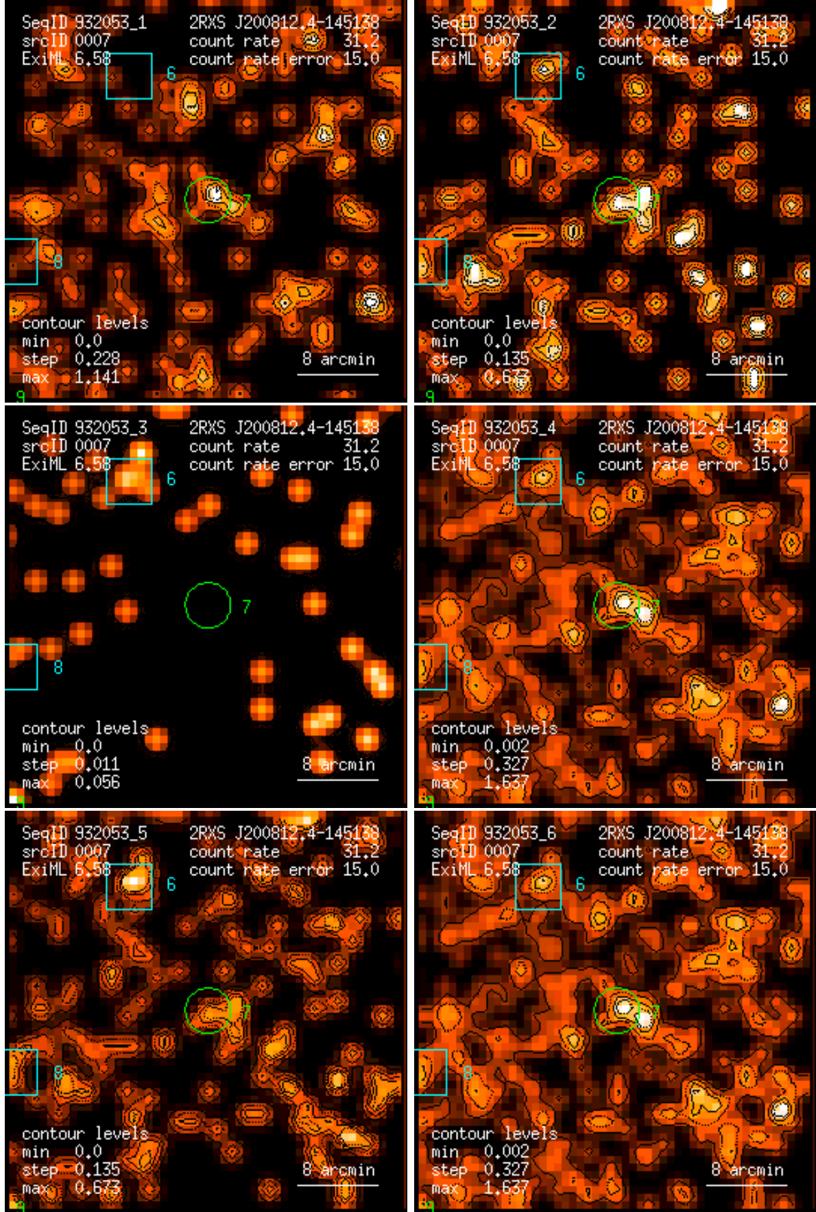
Figure 7: RASS 932053: detection 0007: band rate images, Gaussian filter: (1) PSPC channels 11 – 41, (2) 52 – 90, (3) 91 – 201, (4) 11 – 235, (5) 52 – 201, (6) 11 – 201. Broad band rates in counts/ks. Band rate contour levels in counts/ks/arcmin 2 .
