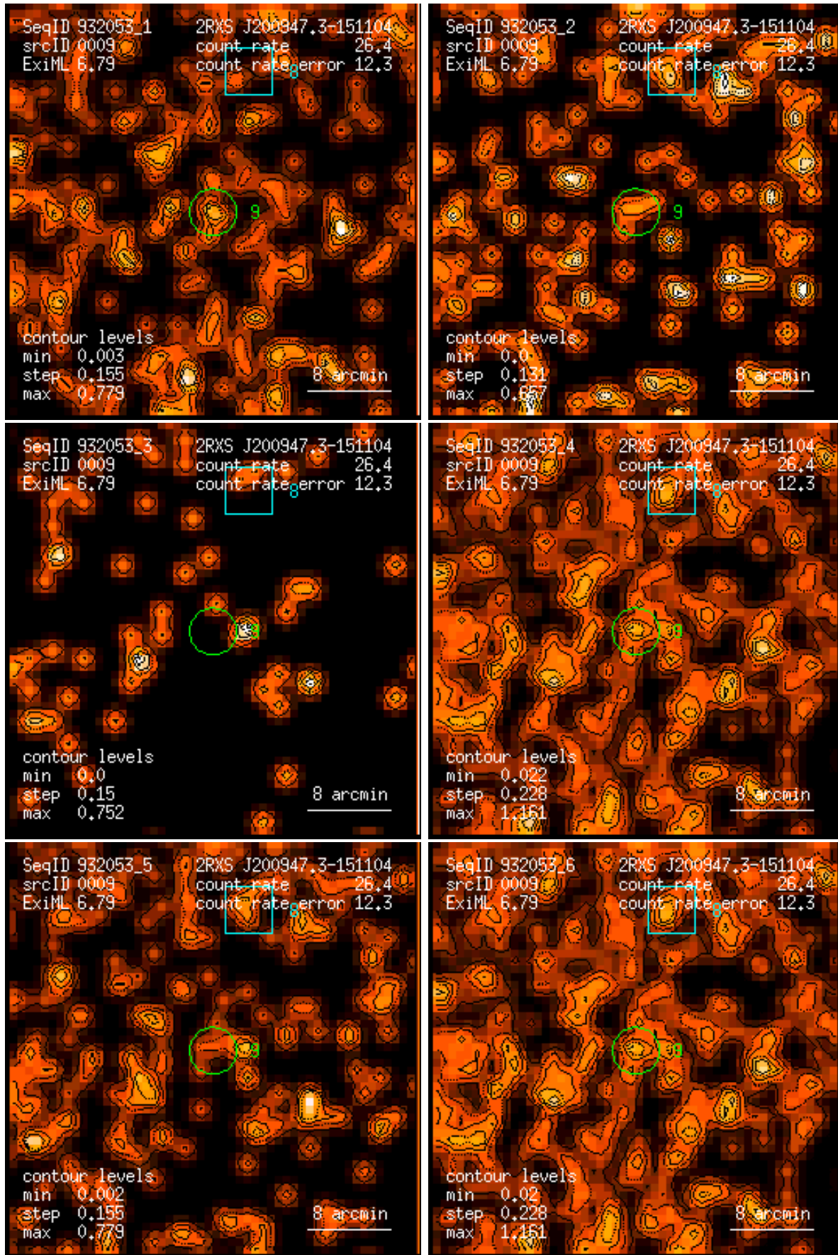
Figure 9: RASS 932053: detection 0009: band rate images, Gaussian filter: (1) PSPC channels 11 – 41, (2) 52 – 90, (3) 91 – 201, (4) 11 – 235, (5) 52 – 201, (6) 11 – 201. Broad band rates in counts/ks. Band rate contour levels in counts/ks/arcmin 2 .
