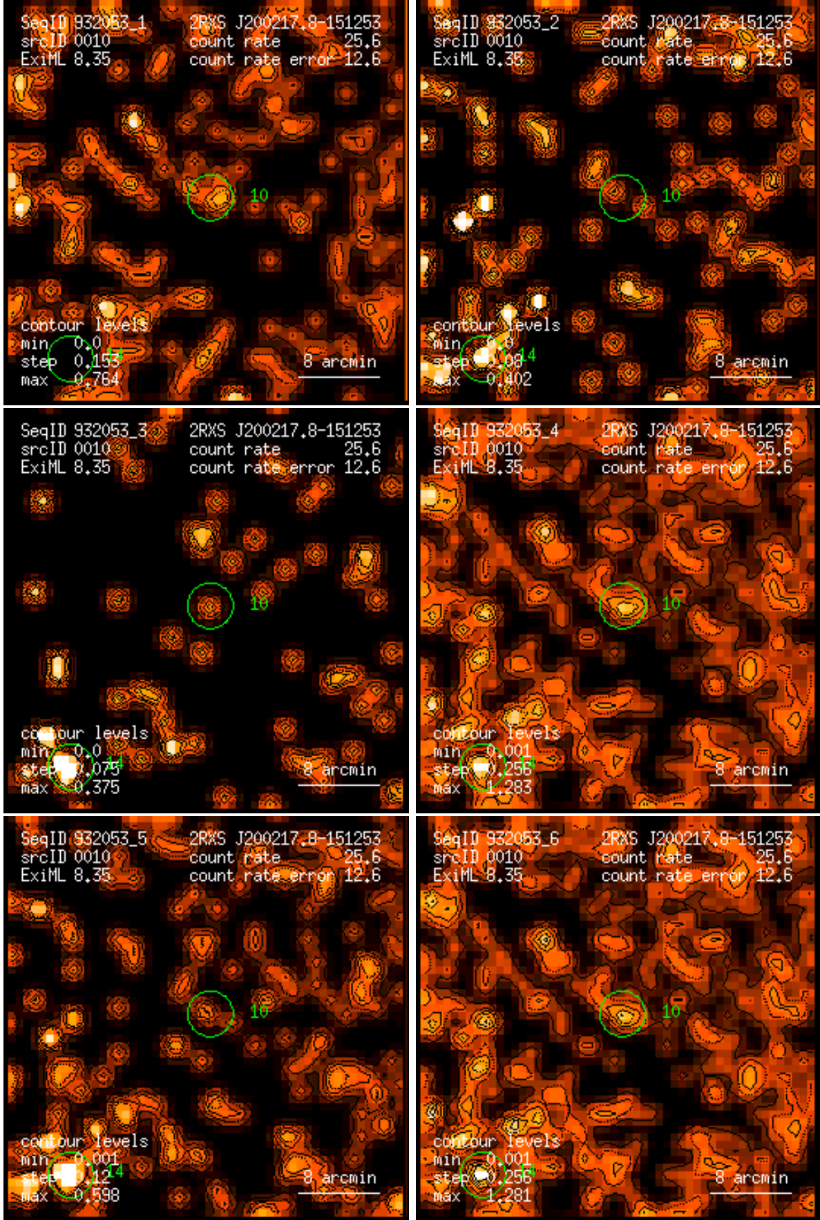
Figure 10: RASS 932053: detection 0010: band rate images, Gaussian filter: (1) PSPC channels 11 – 41, (2) 52 – 90, (3) 91 – 201, (4) 11 – 235, (5) 52 – 201, (6) 11 – 201. Broad band rates in counts/ks. Band rate contour levels in counts/ks/arcmin 2 .
