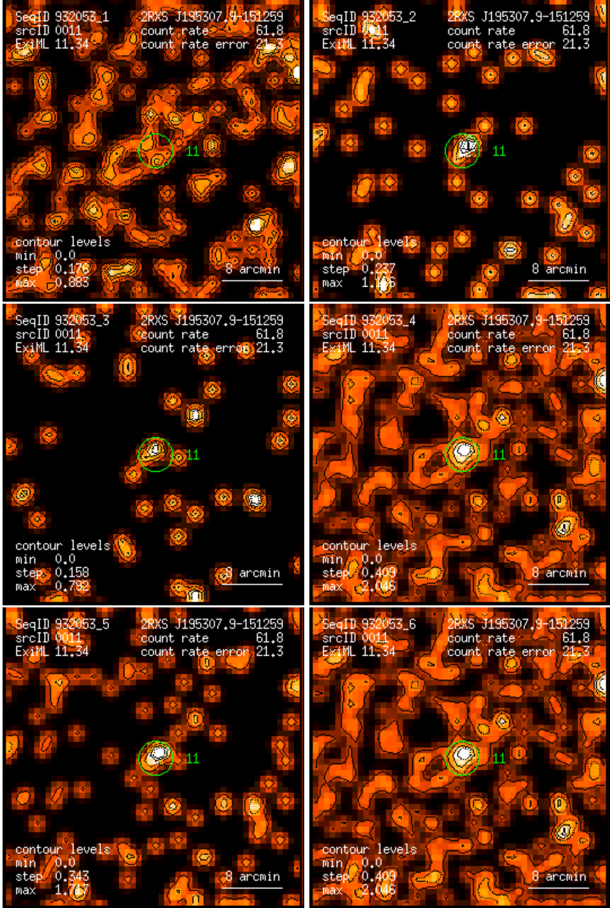
Figure 11: RASS 932053: detection 0011: band rate images, Gaussian filter: (1) PSPC channels 11 – 41, (2) 52 – 90, (3) 91 – 201, (4) 11 – 235, (5) 52 – 201, (6) 11 – 201. Broad band rates in counts/ks. Band rate contour levels in counts/ks/arcmin 2 .
