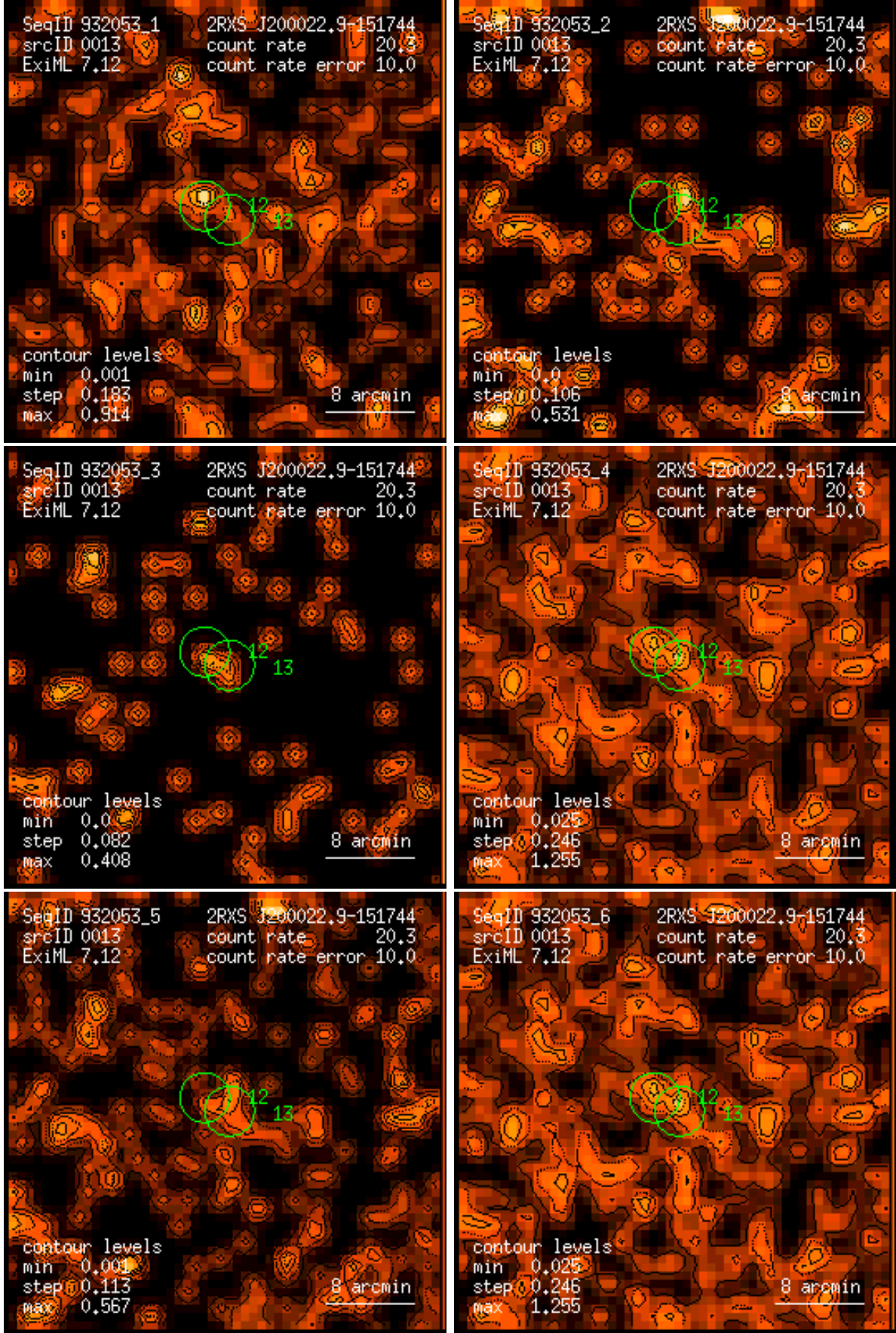
Figure 13: RASS 932053: detection 0013: band rate images, Gaussian filter: (1) PSPC channels 11 – 41, (2) 52 – 90, (3) 91 – 201, (4) 11 – 235, (5) 52 – 201, (6) 11 – 201. Broad band rates in counts/ks. Band rate contour levels in counts/ks/arcmin 2 .
