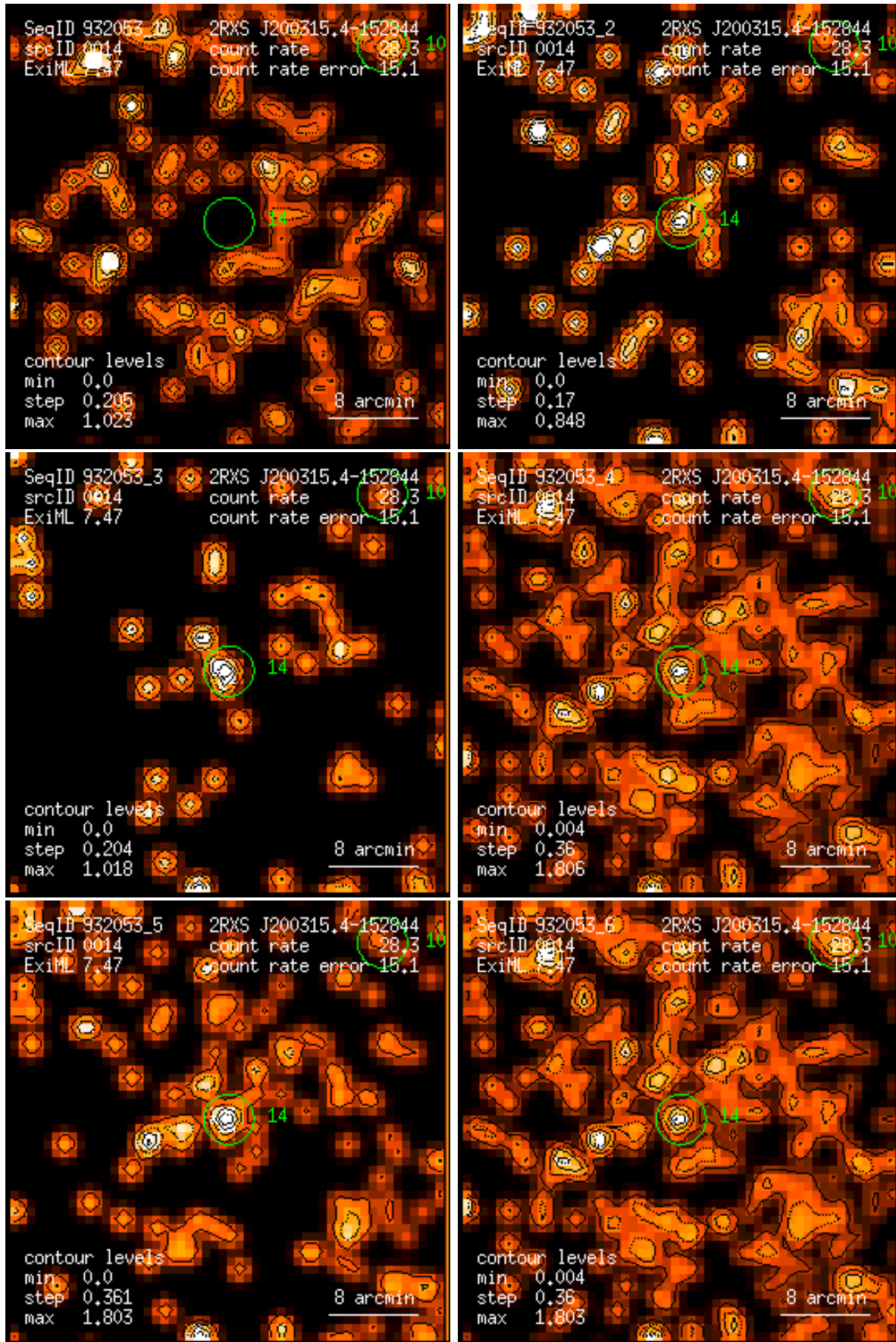
Figure 14: RASS 932053: detection 0014: band rate images, Gaussian filter: (1) PSPC channels 11 – 41, (2) 52 – 90, (3) 91 – 201, (4) 11 – 235, (5) 52 – 201, (6) 11 – 201. Broad band rates in counts/ks. Band rate contour levels in counts/ks/arcmin 2 .
