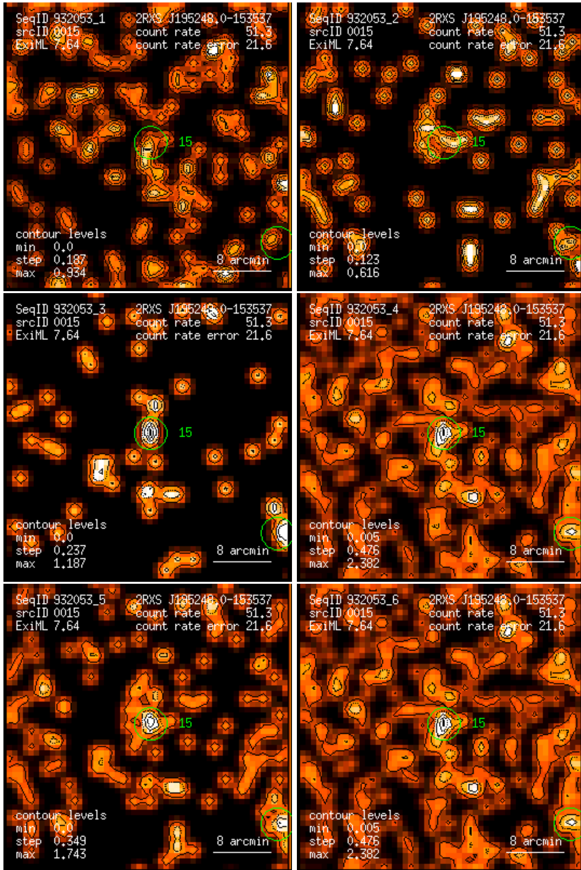
Figure 15: RASS 932053: detection 0015: band rate images, Gaussian filter: (1) PSPC channels 11 – 41, (2) 52 – 90, (3) 91 – 201, (4) 11 – 235, (5) 52 – 201, (6) 11 – 201. Broad band rates in counts/ks. Band rate contour levels in counts/ks/arcmin 2 .
