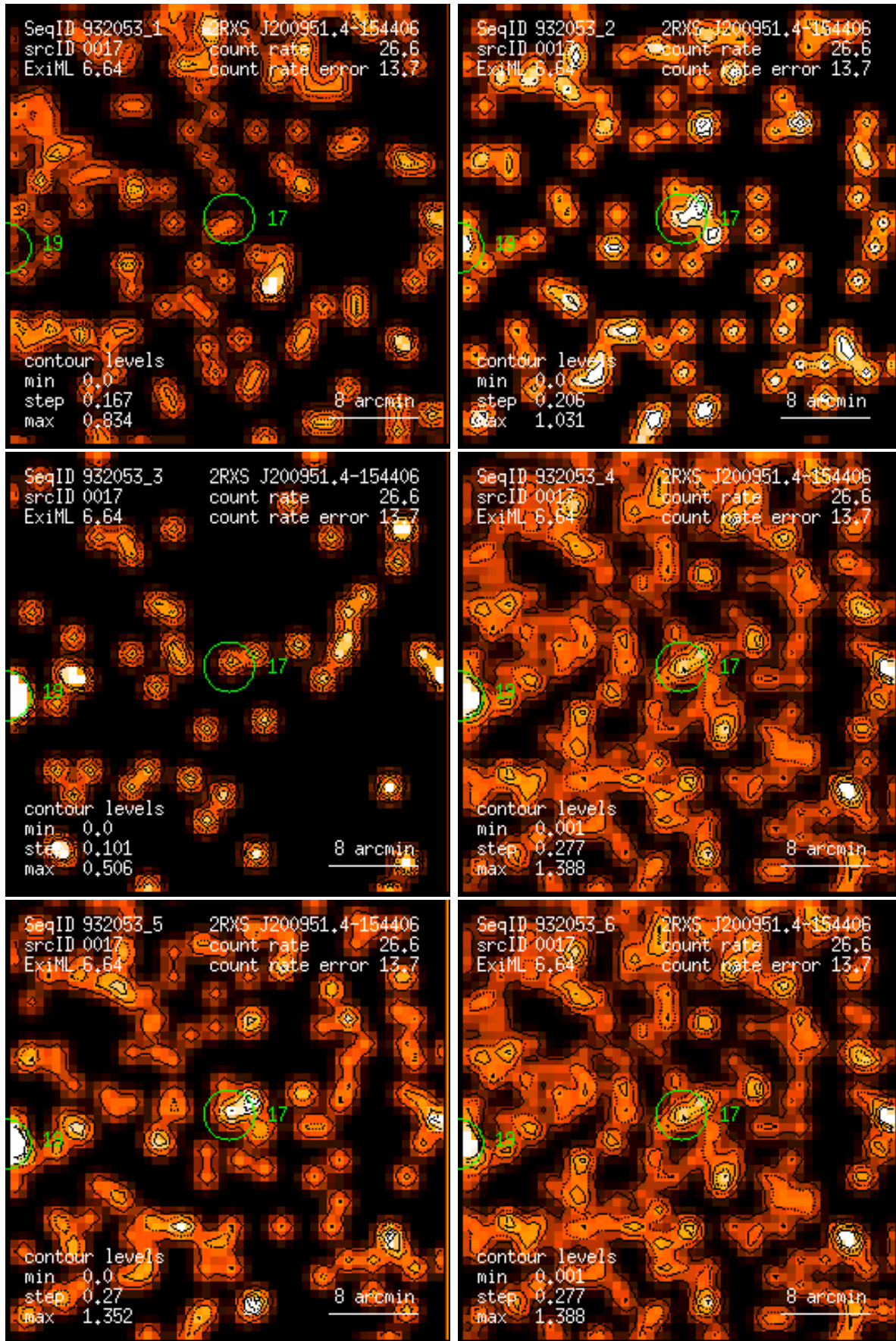
Figure 17: RASS 932053: detection 0017: band rate images, Gaussian filter: (1) PSPC channels 11 – 41, (2) 52 – 90, (3) 91 – 201, (4) 11 – 235, (5) 52 – 201, (6) 11 – 201. Broad band rates in counts/ks. Band rate contour levels in counts/ks/arcmin 2 .
