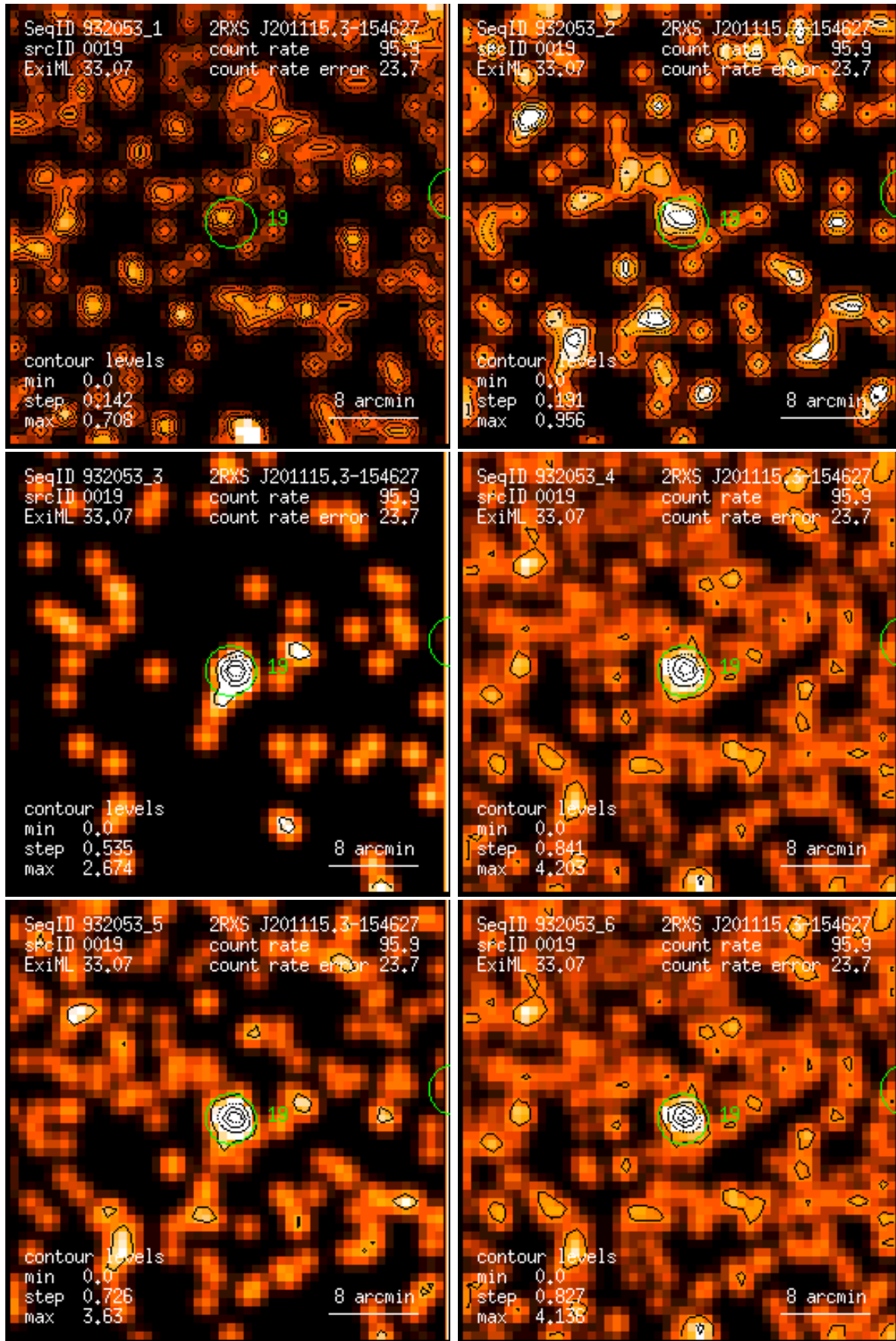
Figure 19: RASS 932053: detection 0019: band rate images, Gaussian filter: (1) PSPC channels 11 – 41, (2) 52 – 90, (3) 91 – 201, (4) 11 – 235, (5) 52 – 201, (6) 11 – 201. Broad band rates in counts/ks. Band rate contour levels in counts/ks/arcmin 2 .
