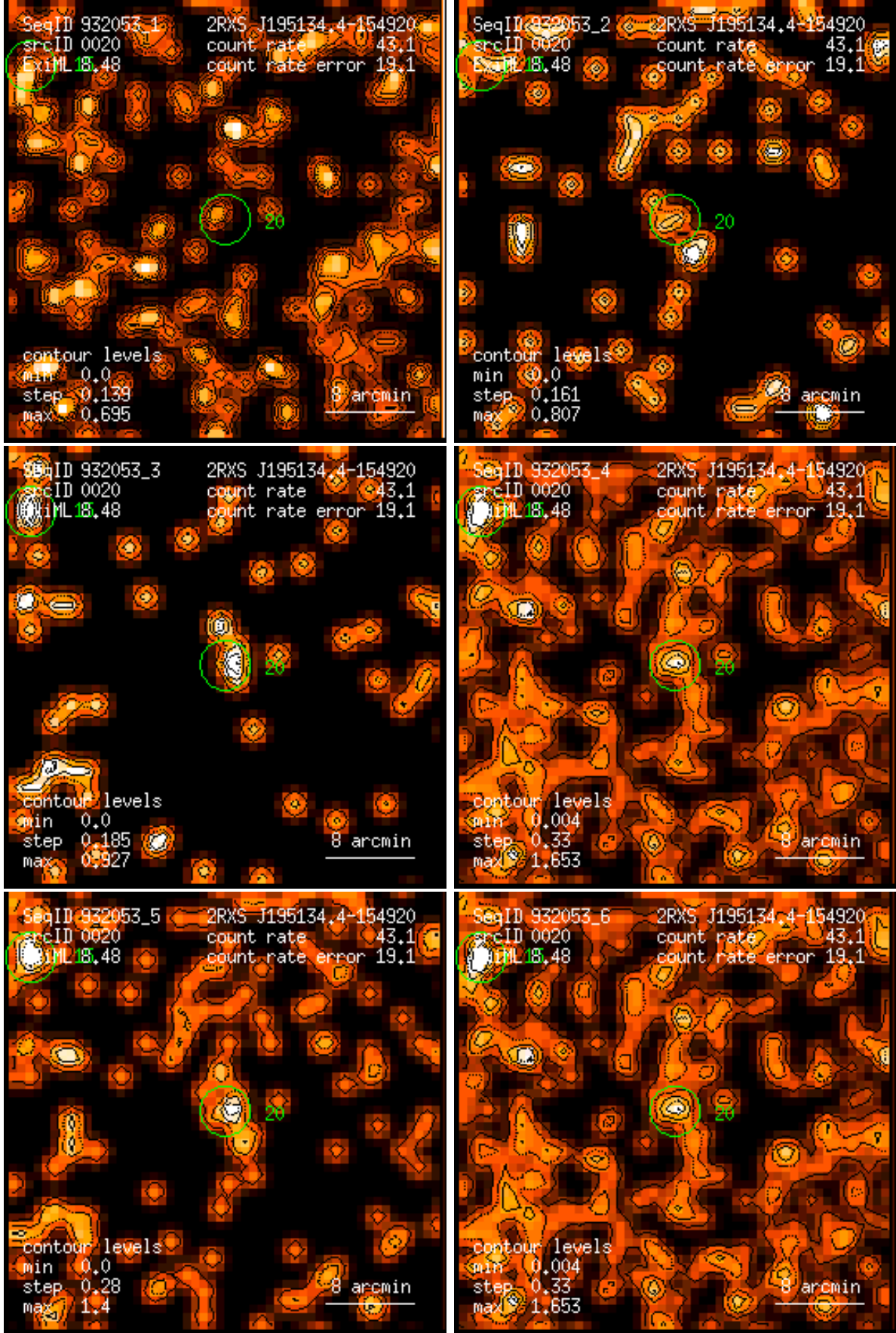
Figure 20: RASS 932053: detection 0020: band rate images, Gaussian filter: (1) PSPC channels 11 – 41, (2) 52 – 90, (3) 91 – 201, (4) 11 – 235, (5) 52 – 201, (6) 11 – 201. Broad band rates in counts/ks. Band rate contour levels in counts/ks/arcmin 2 .
