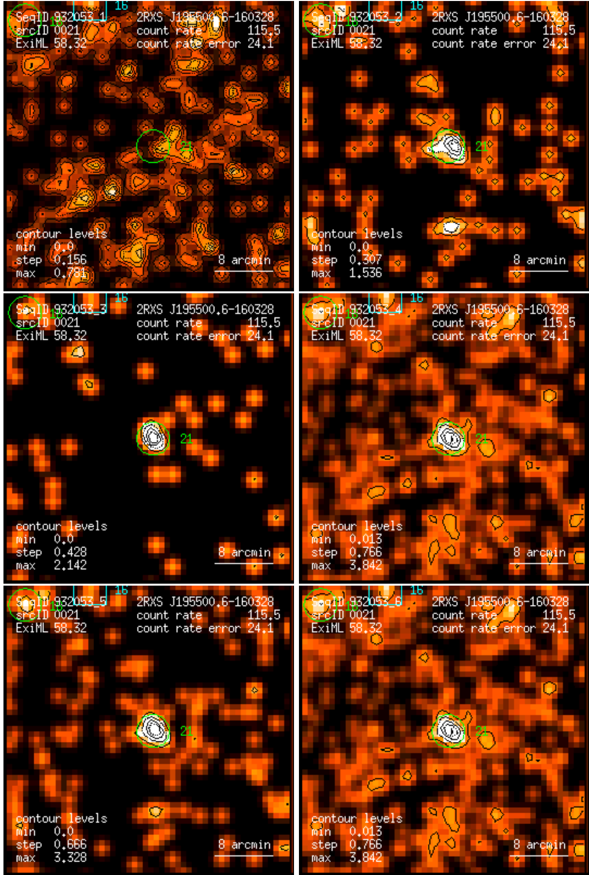
Figure 21: RASS 932053: detection 0021: band rate images, Gaussian filter: (1) PSPC channels 11 – 41, (2) 52 – 90, (3) 91 – 201, (4) 11 – 235, (5) 52 – 201, (6) 11 – 201. Broad band rates in counts/ks. Band rate contour levels in counts/ks/arcmin 2 .
