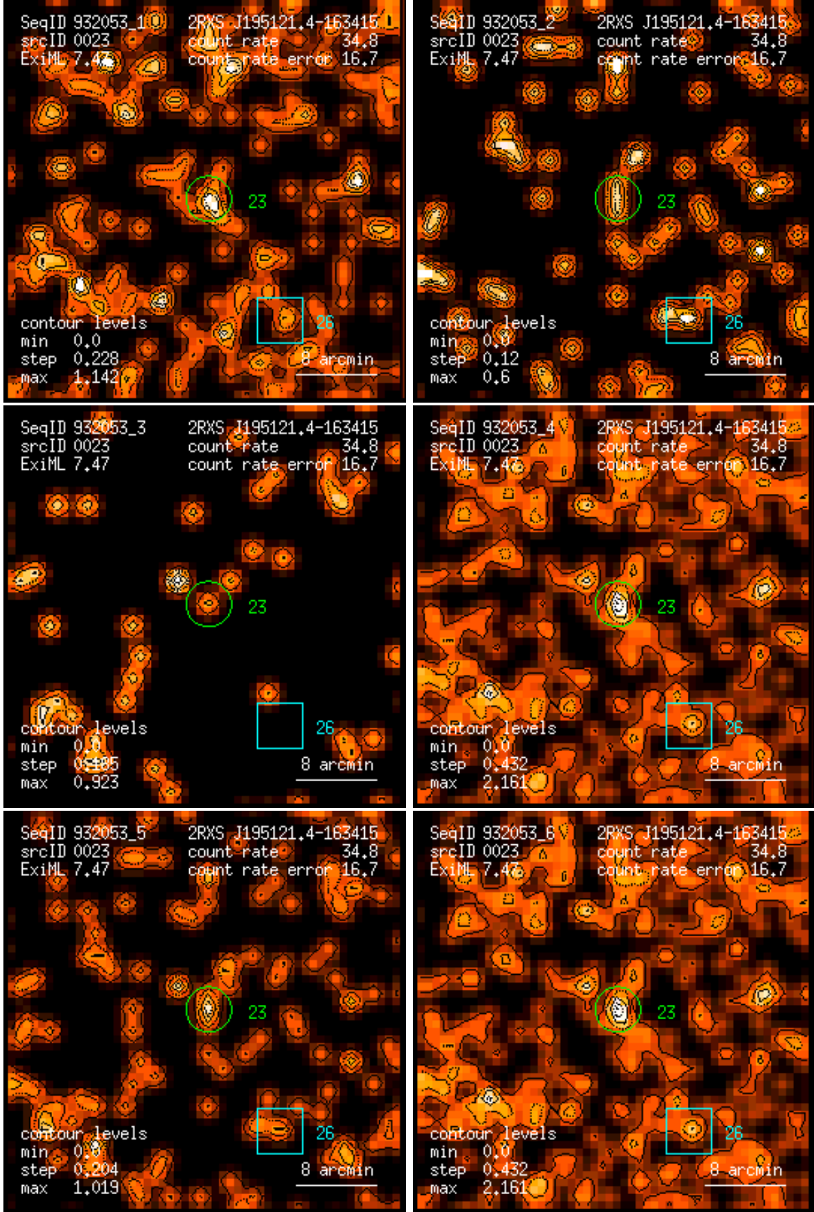
Figure 23: RASS 932053: detection 0023: band rate images, Gaussian filter: (1) PSPC channels 11 – 41, (2) 52 – 90, (3) 91 – 201, (4) 11 – 235, (5) 52 – 201, (6) 11 – 201. Broad band rates in counts/ks. Band rate contour levels in counts/ks/arcmin 2 .
