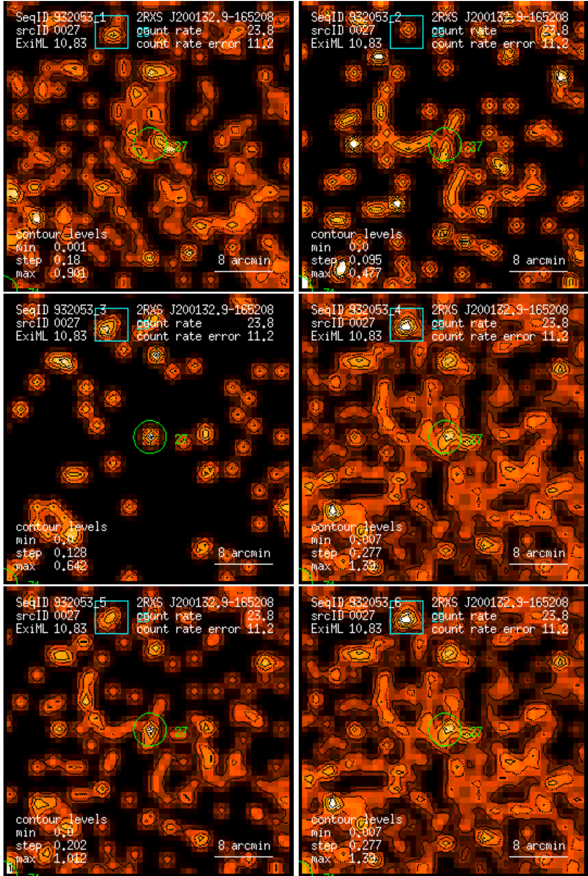
Figure 27: RASS 932053: detection 0027: band rate images, Gaussian filter: (1) PSPC channels 11 – 41, (2) 52 – 90, (3) 91 – 201, (4) 11 – 235, (5) 52 – 201, (6) 11 – 201. Broad band rates in counts/ks. Band rate contour levels in counts/ks/arcmin 2 .
