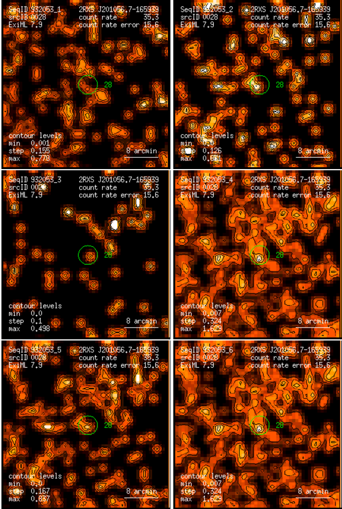
Figure 28: RASS 932053: detection 0028: band rate images, Gaussian filter: (1) PSPC channels 11 – 41, (2) 52 – 90, (3) 91 – 201, (4) 11 – 235, (5) 52 – 201, (6) 11 – 201. Broad band rates in counts/ks. Band rate contour levels in counts/ks/arcmin 2 .
