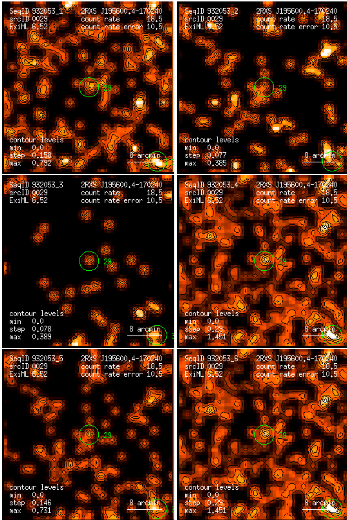
Figure 29: RASS 932053: detection 0029: band rate images, Gaussian filter: (1) PSPC channels 11 – 41, (2) 52 – 90, (3) 91 – 201, (4) 11 – 235, (5) 52 – 201, (6) 11 – 201. Broad band rates in counts/ks. Band rate contour levels in counts/ks/arcmin 2 .
