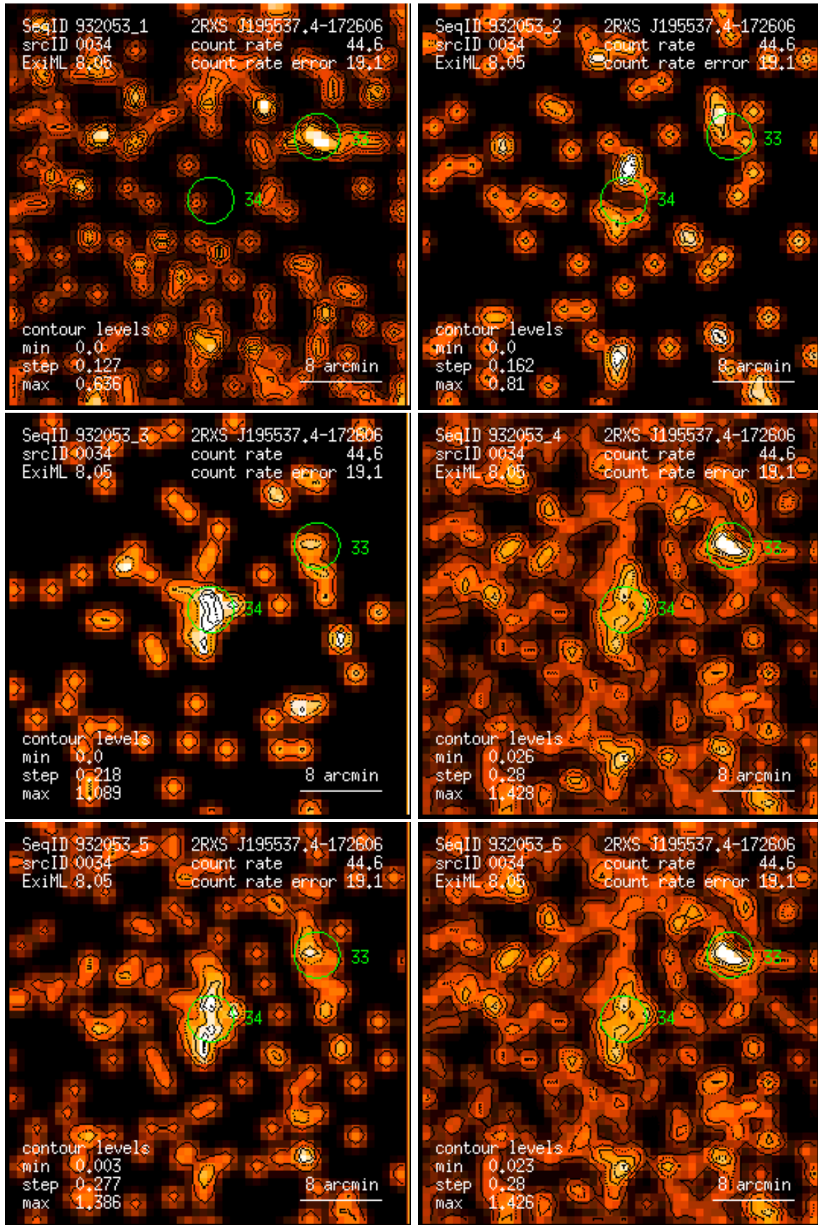
Figure 34: RASS 932053: detection 0034: band rate images, Gaussian filter: (1) PSPC channels 11 – 41, (2) 52 – 90, (3) 91 – 201, (4) 11 – 235, (5) 52 – 201, (6) 11 – 201. Broad band rates in counts/ks. Band rate contour levels in counts/ks/arcmin 2 .
