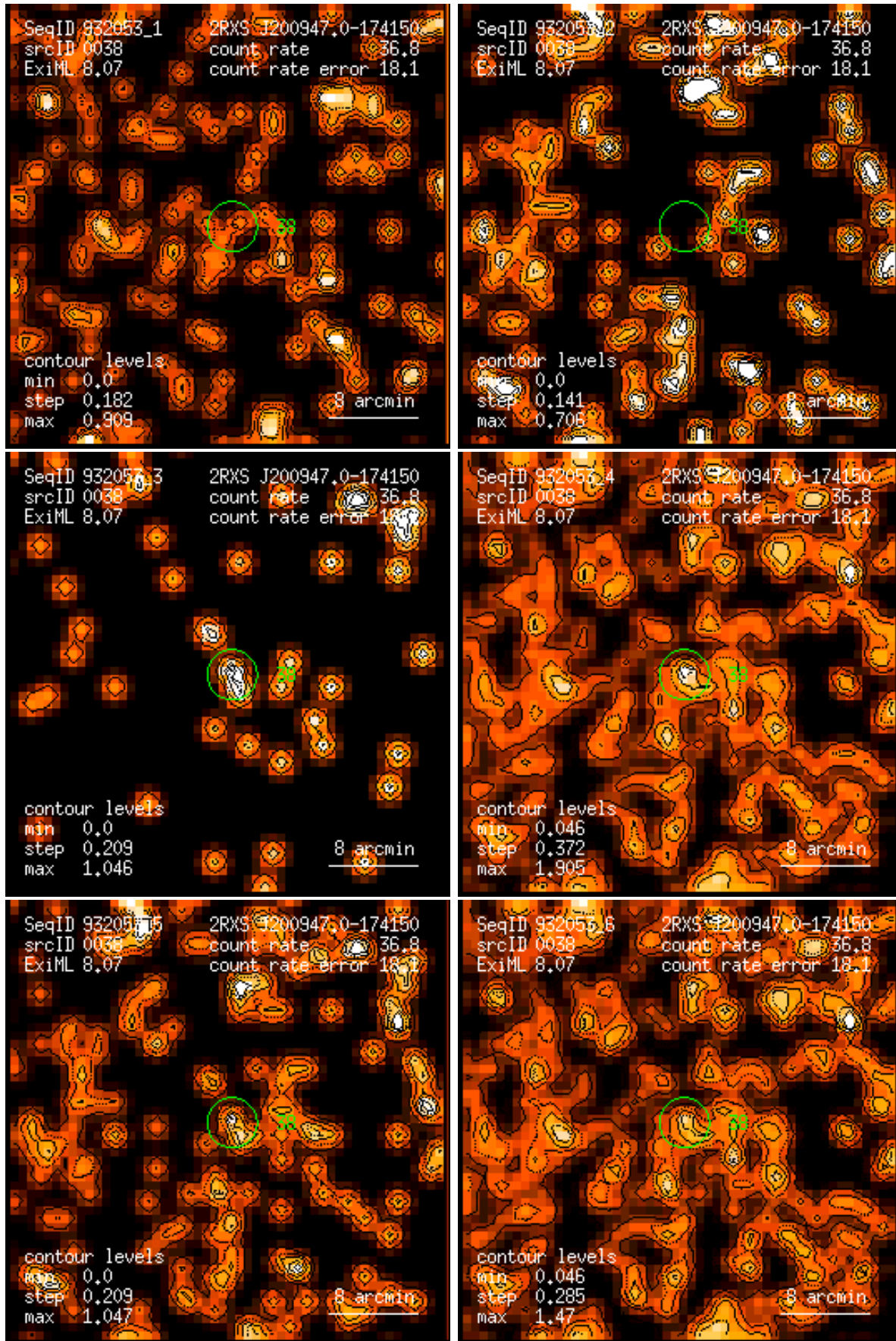
Figure 38: RASS 932053: detection 0038: band rate images, Gaussian filter: (1) PSPC channels 11 – 41, (2) 52 – 90, (3) 91 – 201, (4) 11 – 235, (5) 52 – 201, (6) 11 – 201. Broad band rates in counts/ks. Band rate contour levels in counts/ks/arcmin 2 .
