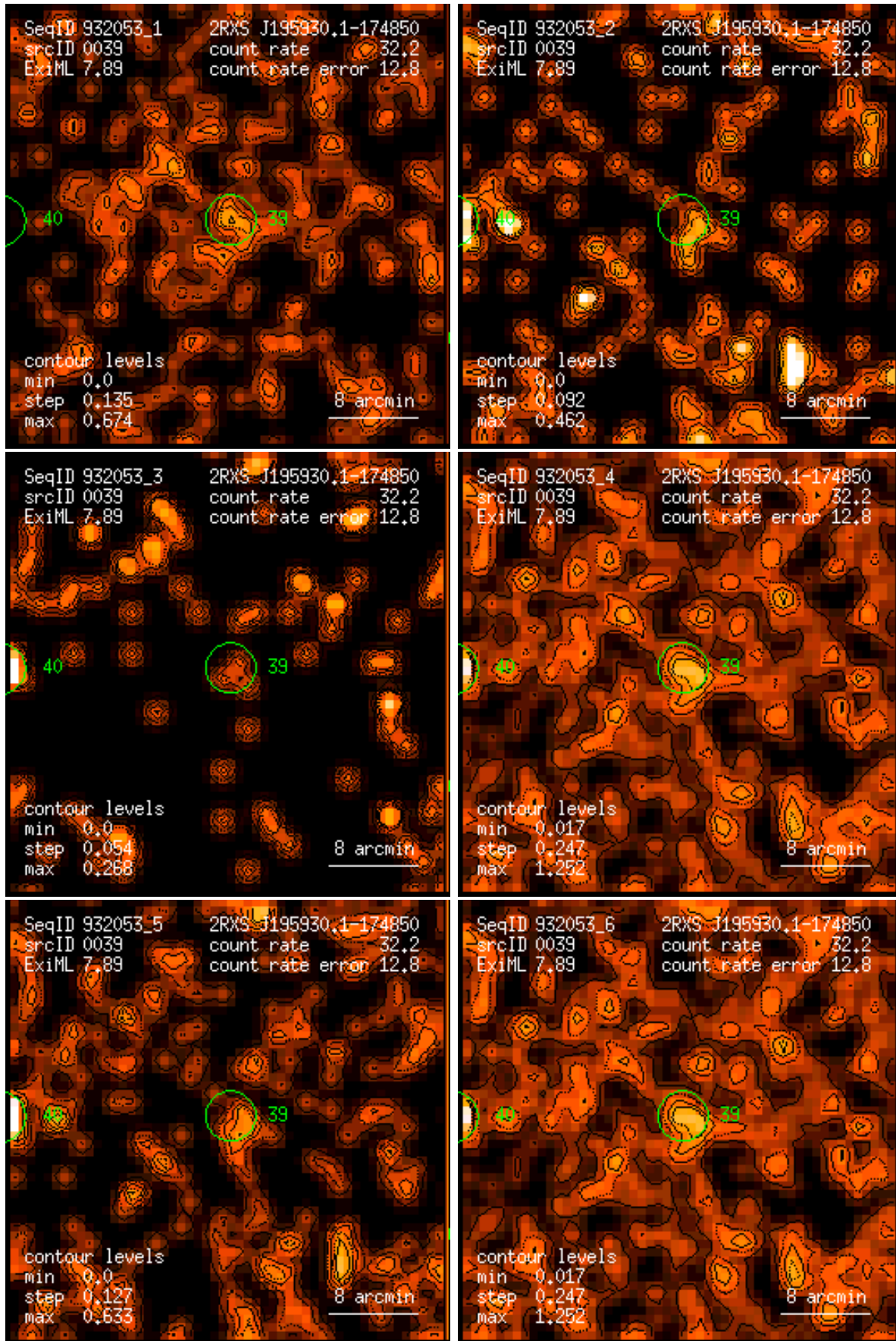
Figure 39: RASS 932053: detection 0039: band rate images, Gaussian filter: (1) PSPC channels 11 – 41, (2) 52 – 90, (3) 91 – 201, (4) 11 – 235, (5) 52 – 201, (6) 11 – 201. Broad band rates in counts/ks. Band rate contour levels in counts/ks/arcmin 2 .
