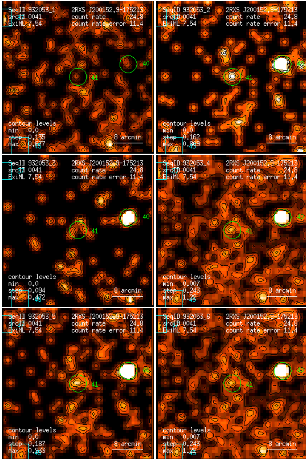
Figure 41: RASS 932053: detection 0041: band rate images, Gaussian filter: (1) PSPC channels 11 – 41, (2) 52 – 90, (3) 91 – 201, (4) 11 – 235, (5) 52 – 201, (6) 11 – 201. Broad band rates in counts/ks. Band rate contour levels in counts/ks/arcmin 2 .
