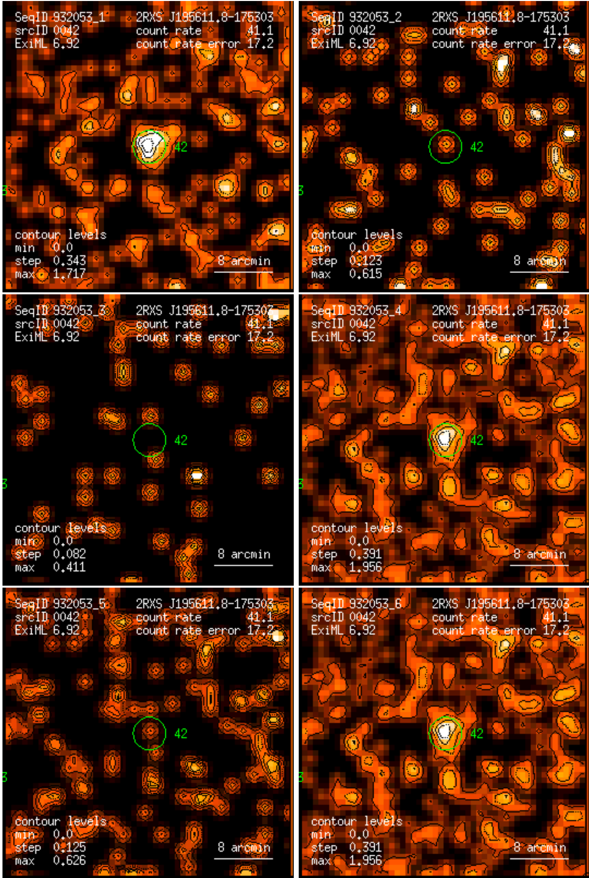
Figure 42: RASS 932053: detection 0042: band rate images, Gaussian filter: (1) PSPC channels 11 – 41, (2) 52 – 90, (3) 91 – 201, (4) 11 – 235, (5) 52 – 201, (6) 11 – 201. Broad band rates in counts/ks. Band rate contour levels in counts/ks/arcmin 2 .
