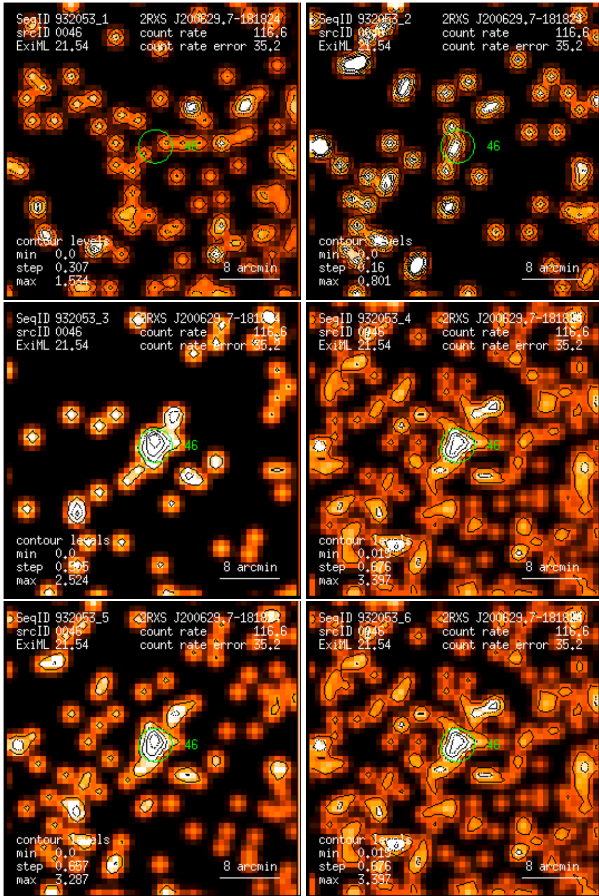
Figure 46: RASS 932053: detection 0046: band rate images, Gaussian filter: (1) PSPC channels 11 – 41, (2) 52 – 90, (3) 91 – 201, (4) 11 – 235, (5) 52 – 201, (6) 11 – 201. Broad band rates in counts/ks. Band rate contour levels in counts/ks/arcmin 2 .
