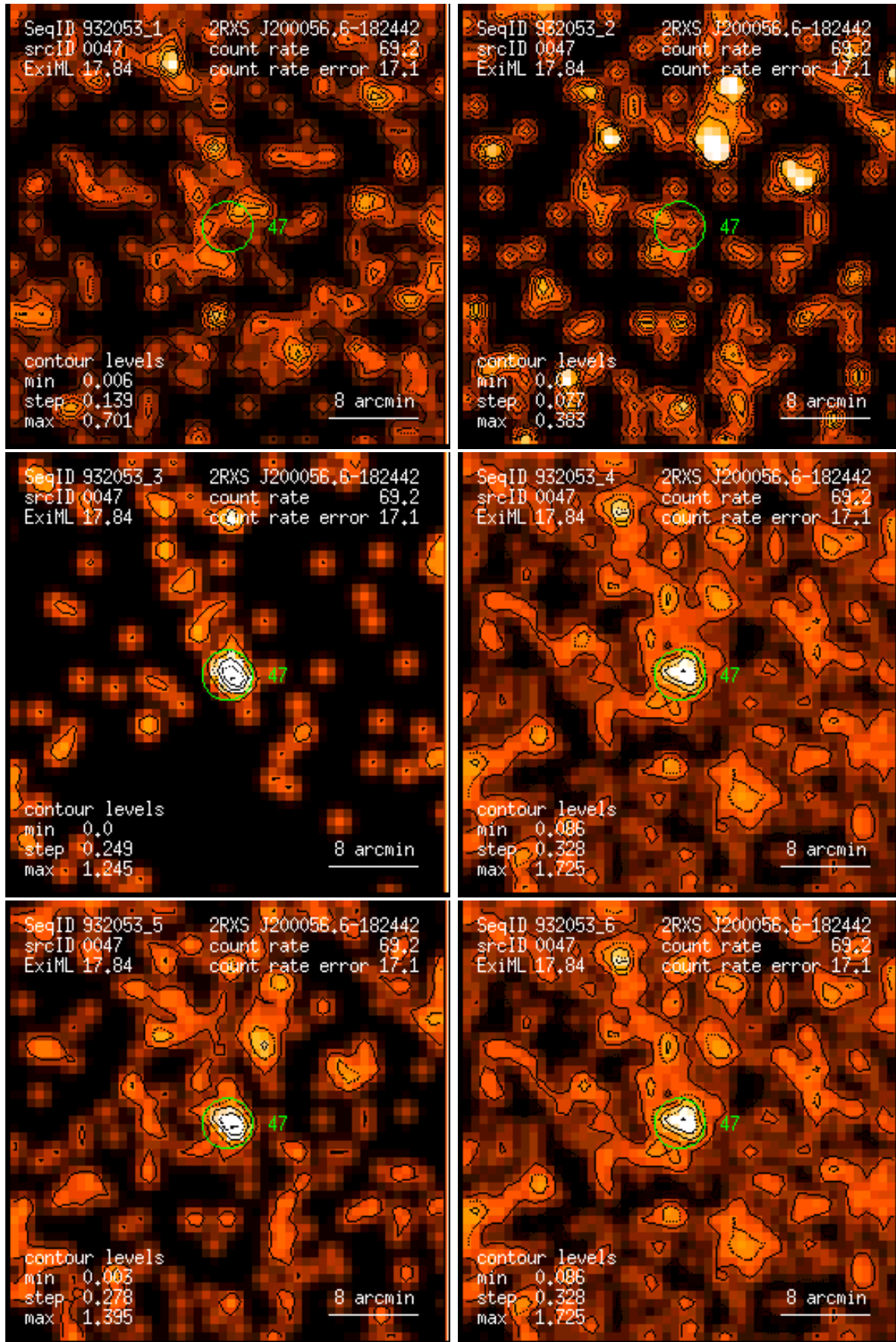
Figure 47: RASS 932053: detection 0047: band rate images, Gaussian filter: (1) PSPC channels 11 – 41, (2) 52 – 90, (3) 91 – 201, (4) 11 – 235, (5) 52 – 201, (6) 11 – 201. Broad band rates in counts/ks. Band rate contour levels in counts/ks/arcmin 2 .
