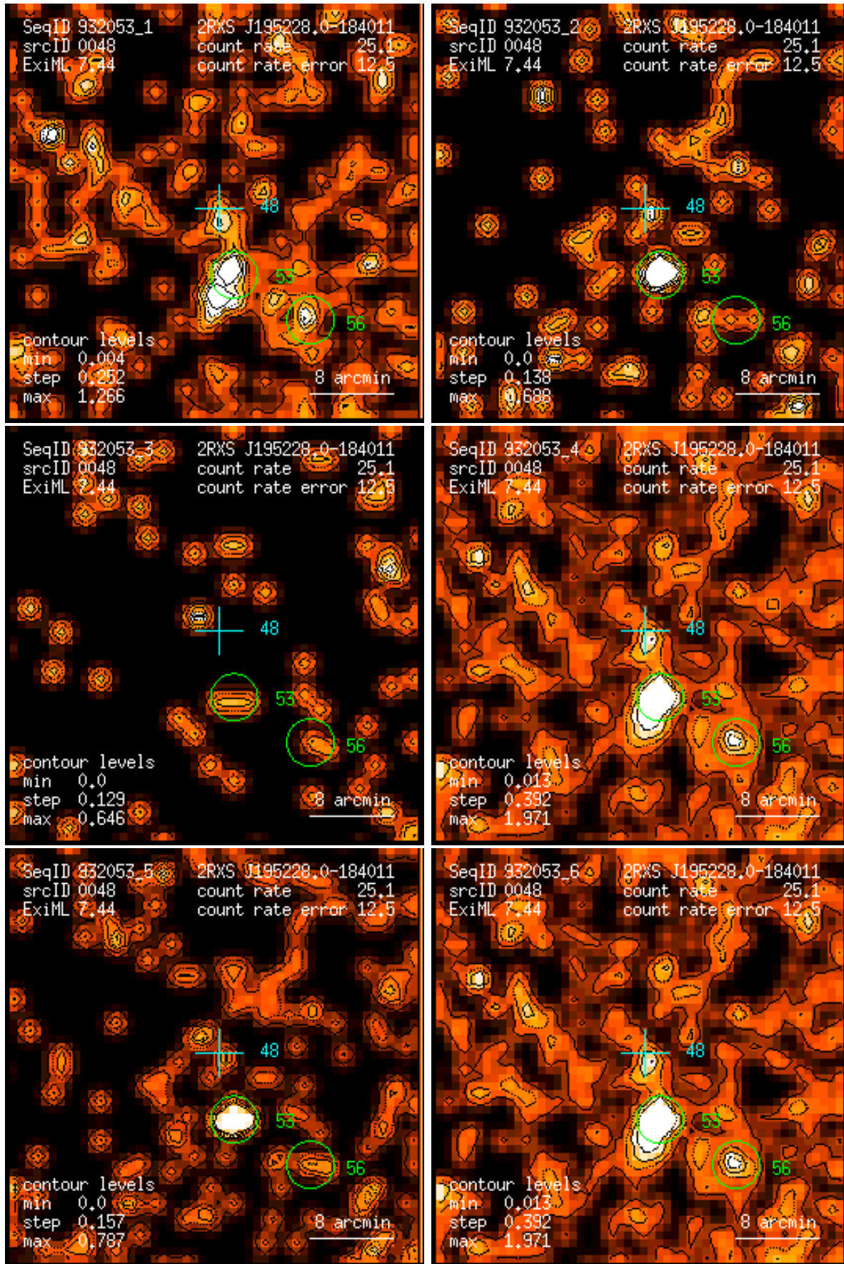
Figure 48: RASS 932053: detection 0048: band rate images, Gaussian filter: (1) PSPC channels 11 – 41, (2) 52 – 90, (3) 91 – 201, (4) 11 – 235, (5) 52 – 201, (6) 11 – 201. Broad band rates in counts/ks. Band rate contour levels in counts/ks/arcmin 2 .
