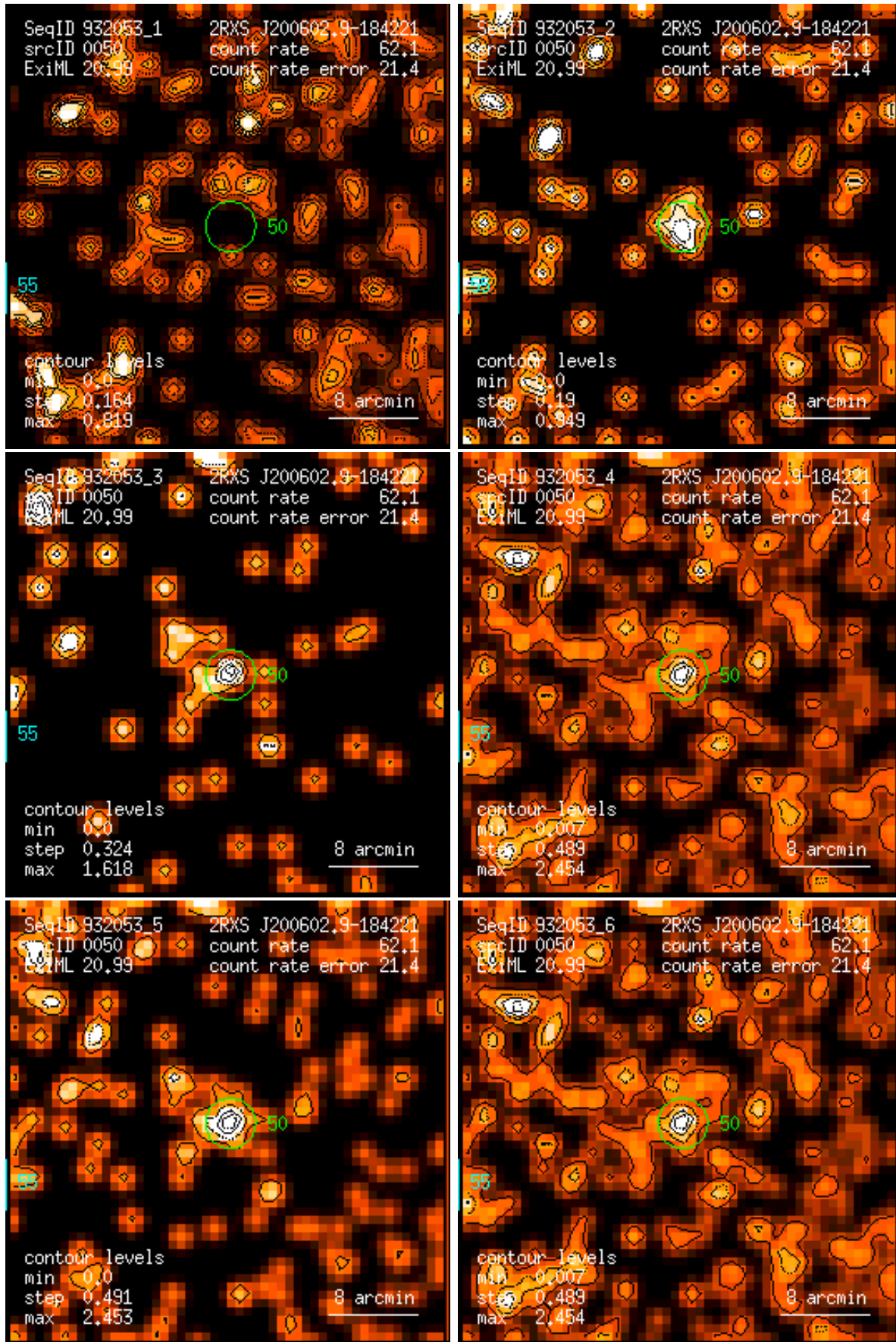
Figure 50: RASS 932053: detection 0050: band rate images, Gaussian filter: (1) PSPC channels 11 – 41, (2) 52 – 90, (3) 91 – 201, (4) 11 – 235, (5) 52 – 201, (6) 11 – 201. Broad band rates in counts/ks. Band rate contour levels in counts/ks/arcmin 2 .
