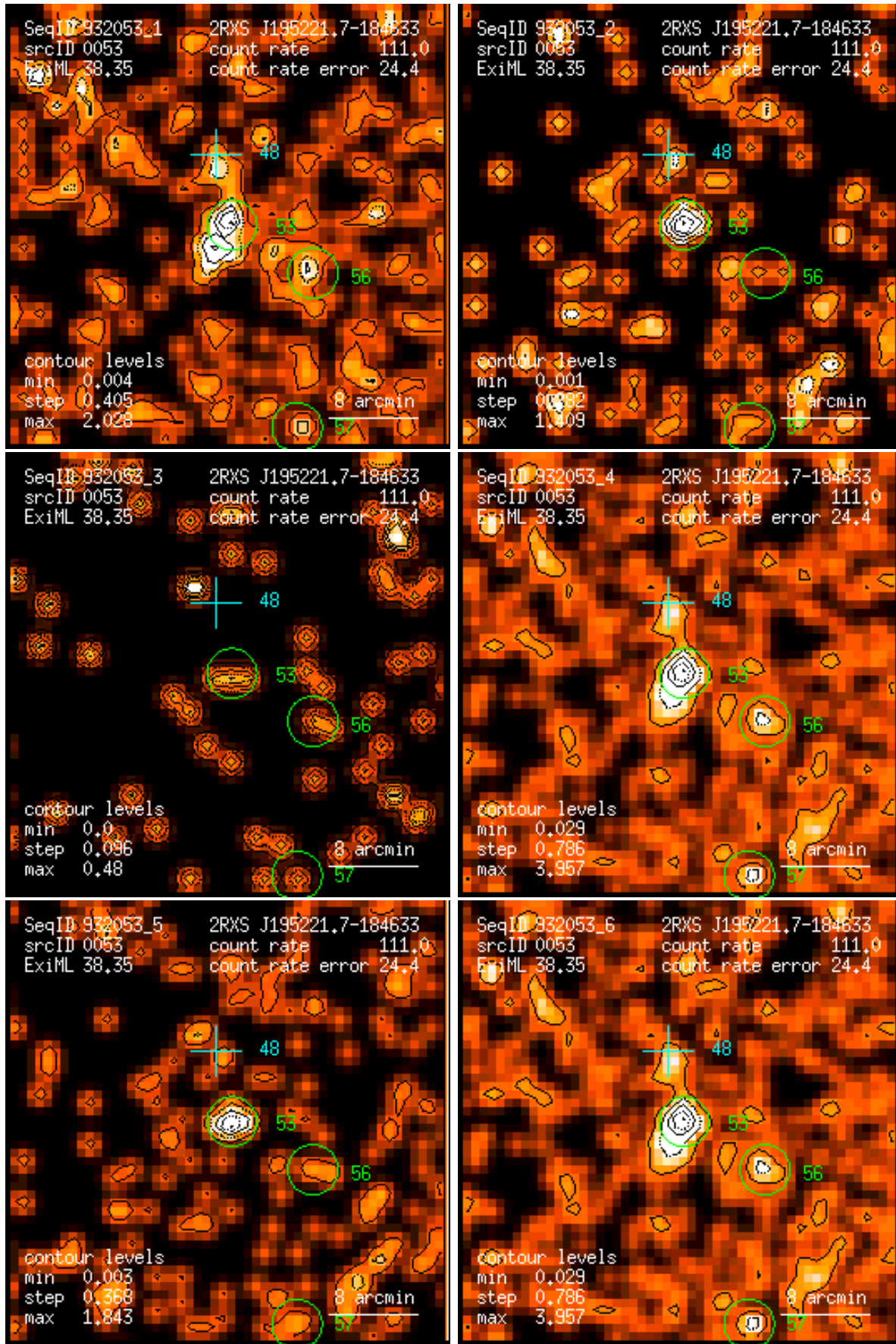
Figure 53: RASS 932053: detection 0053: band rate images, Gaussian filter: (1) PSPC channels 11 – 41, (2) 52 – 90, (3) 91 – 201, (4) 11 – 235, (5) 52 – 201, (6) 11 – 201. Broad band rates in counts/ks. Band rate contour levels in counts/ks/arcmin 2 .
