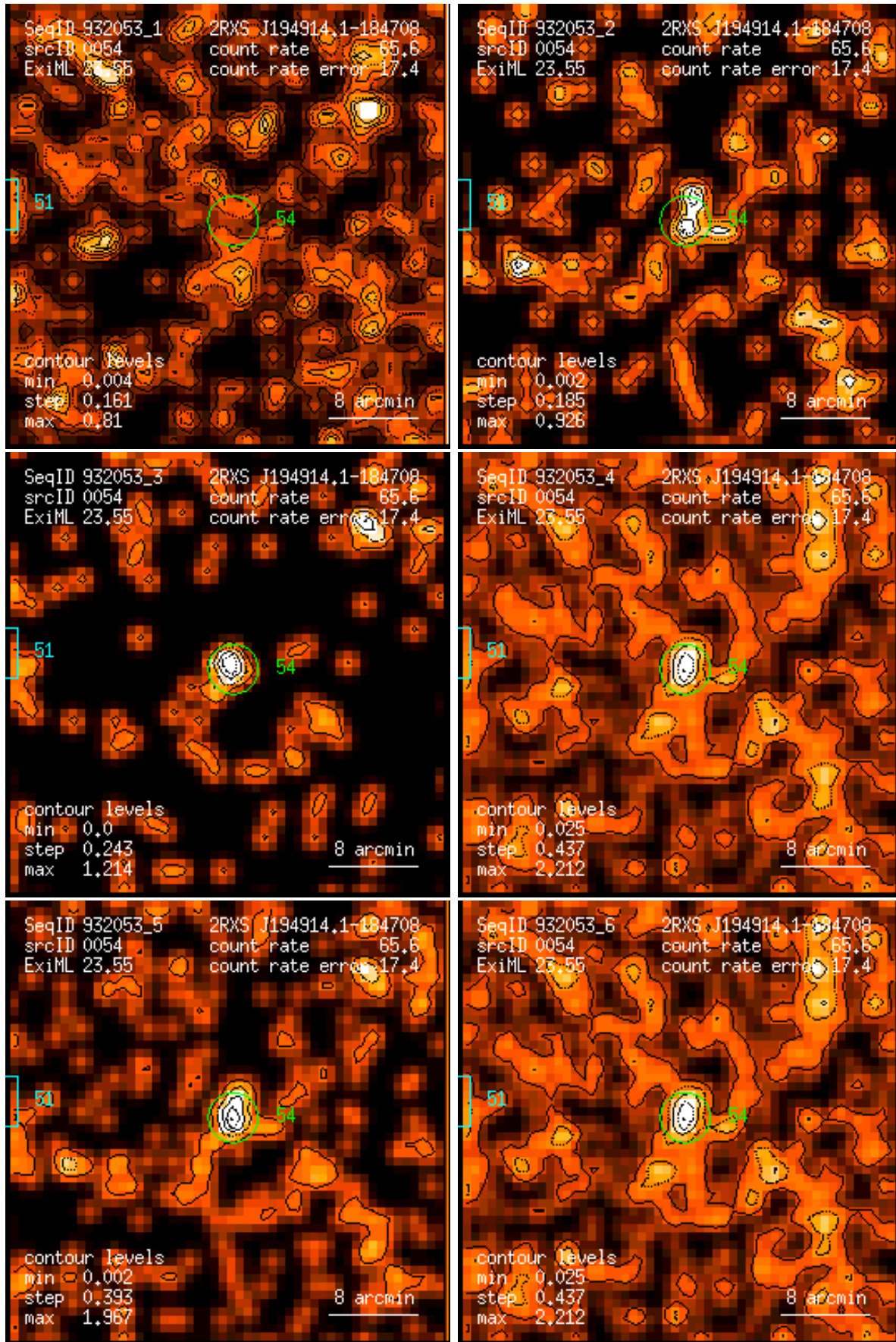
Figure 54: RASS 932053: detection 0054: band rate images, Gaussian filter: (1) PSPC channels 11 – 41, (2) 52 – 90, (3) 91 – 201, (4) 11 – 235, (5) 52 – 201, (6) 11 – 201. Broad band rates in counts/ks. Band rate contour levels in counts/ks/arcmin 2 .
