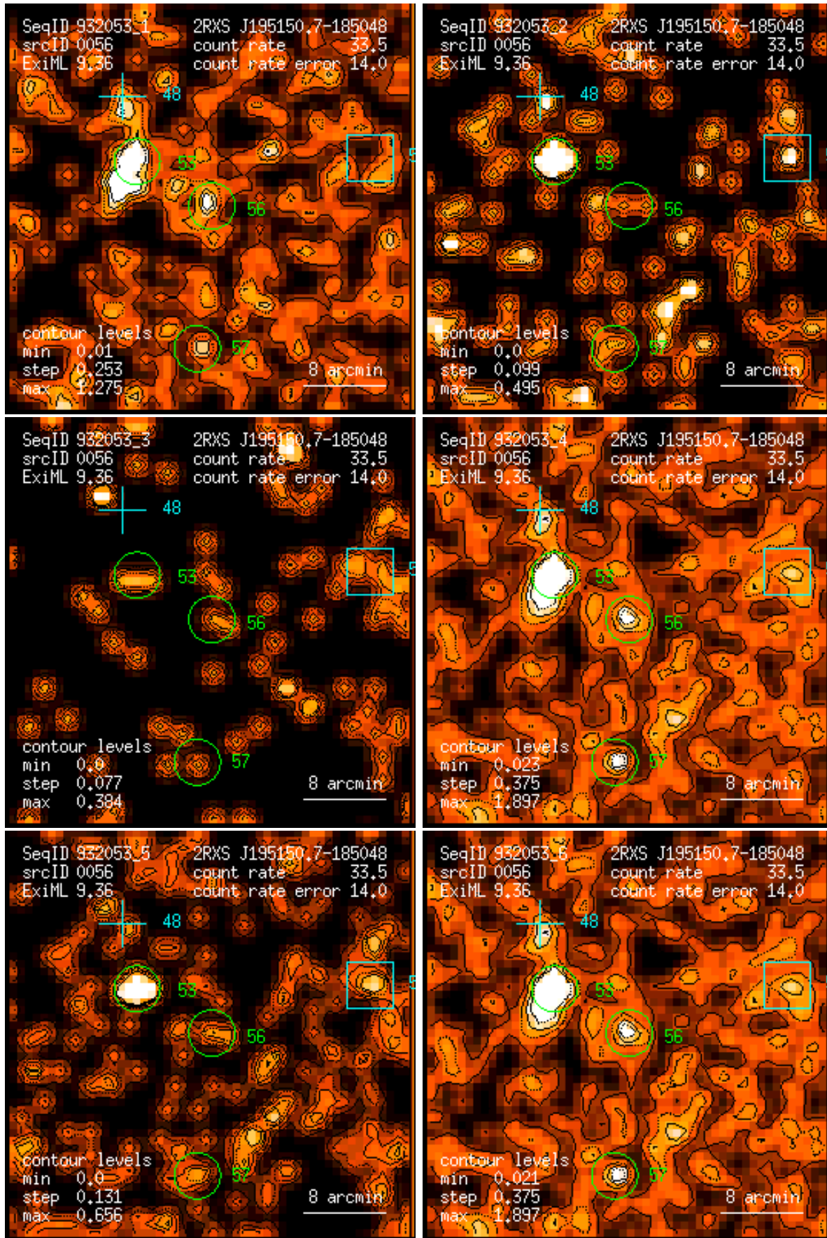
Figure 56: RASS 932053: detection 0056: band rate images, Gaussian filter: (1) PSPC channels 11 – 41, (2) 52 – 90, (3) 91 – 201, (4) 11 – 235, (5) 52 – 201, (6) 11 – 201. Broad band rates in counts/ks. Band rate contour levels in counts/ks/arcmin 2 .
