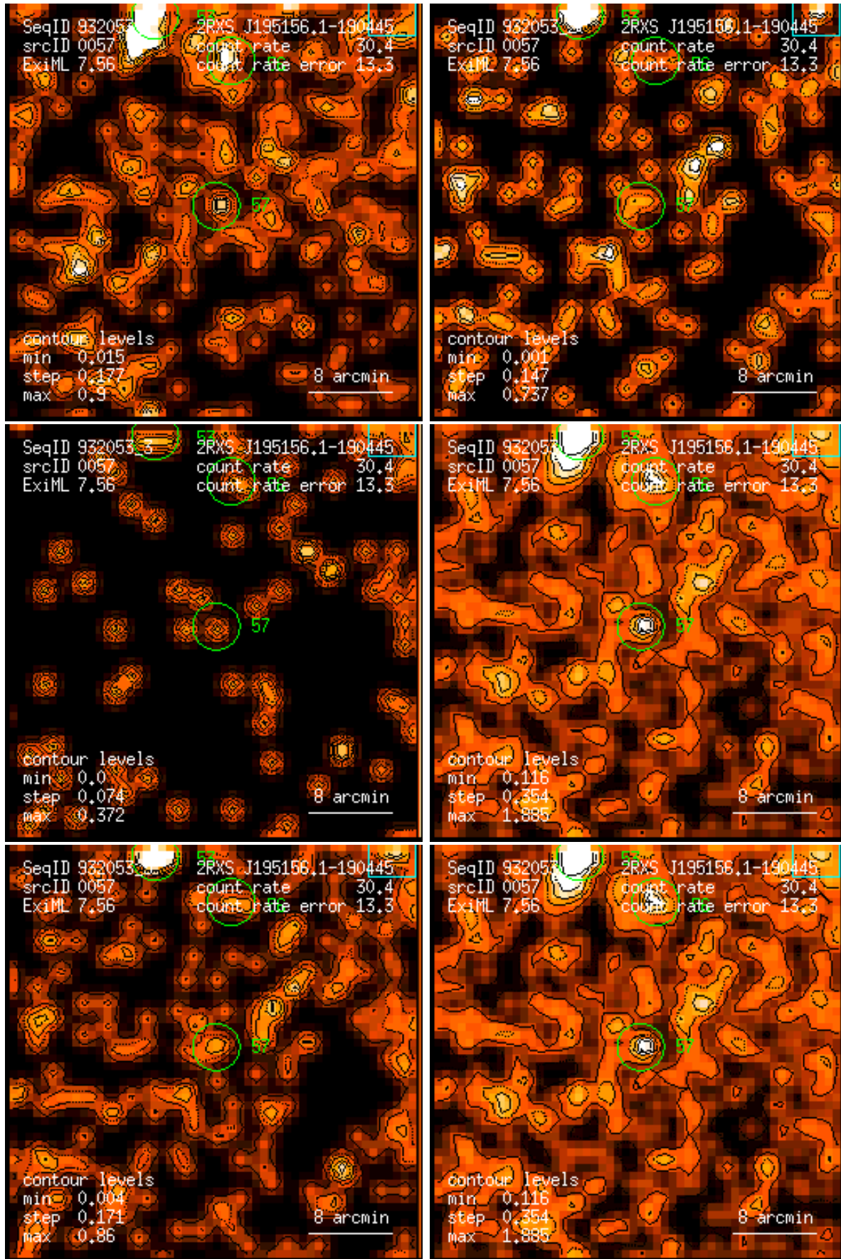
Figure 57: RASS 932053: detection 0057: band rate images, Gaussian filter: (1) PSPC channels 11 – 41, (2) 52 – 90, (3) 91 – 201, (4) 11 – 235, (5) 52 – 201, (6) 11 – 201. Broad band rates in counts/ks. Band rate contour levels in counts/ks/arcmin 2 .
