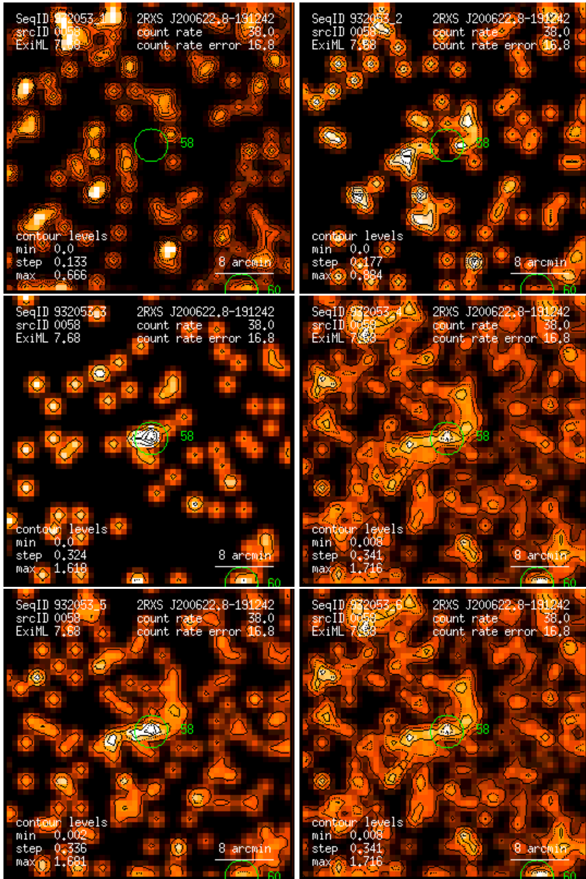
Figure 58: RASS 932053: detection 0058: band rate images, Gaussian filter: (1) PSPC channels 11 – 41, (2) 52 – 90, (3) 91 – 201, (4) 11 – 235, (5) 52 – 201, (6) 11 – 201. Broad band rates in counts/ks. Band rate contour levels in counts/ks/arcmin 2 .
