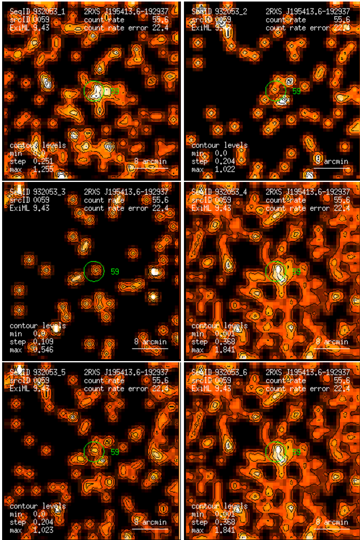
Figure 59: RASS 932053: detection 0059: band rate images, Gaussian filter: (1) PSPC channels 11 – 41, (2) 52 – 90, (3) 91 – 201, (4) 11 – 235, (5) 52 – 201, (6) 11 – 201. Broad band rates in counts/ks. Band rate contour levels in counts/ks/arcmin 2 .
