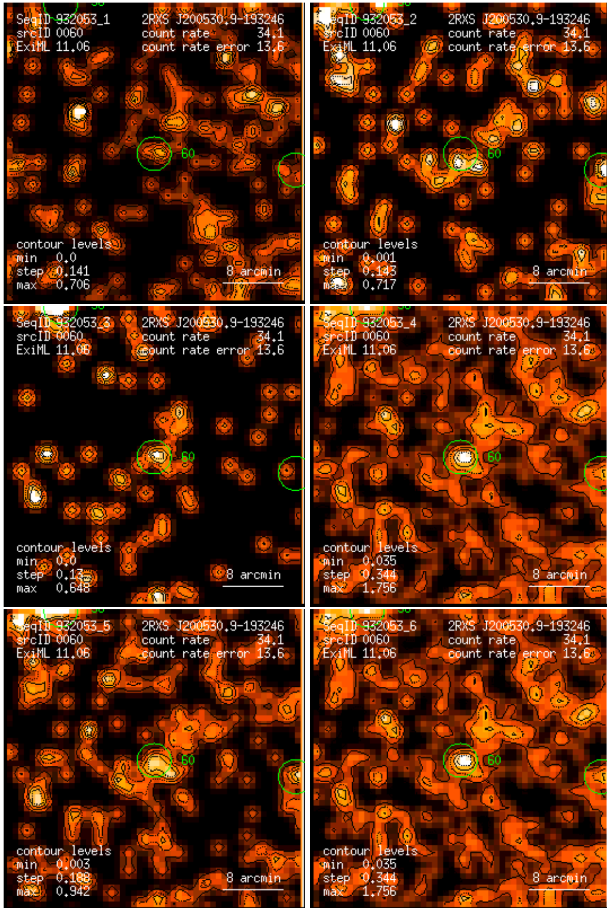
Figure 60: RASS 932053: detection 0060: band rate images, Gaussian filter: (1) PSPC channels 11 – 41, (2) 52 – 90, (3) 91 – 201, (4) 11 – 235, (5) 52 – 201, (6) 11 – 201. Broad band rates in counts/ks. Band rate contour levels in counts/ks/arcmin 2 .
