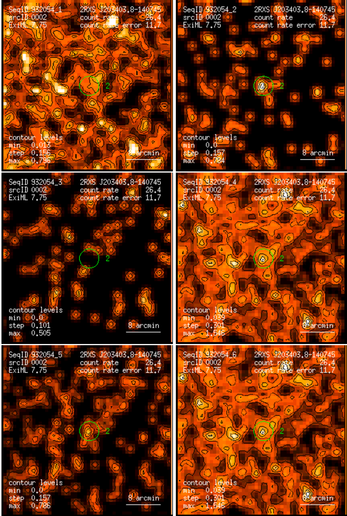
Figure 2: RASS 932054: detection 0002: band rate images, Gaussian filter: (1) PSPC channels 11 – 41, (2) 52 – 90, (3) 91 – 201, (4) 11 – 235, (5) 52 – 201, (6) 11 – 201. Broad band rates in counts/ks. Band rate contour levels in counts/ks/arcmin 2 .
