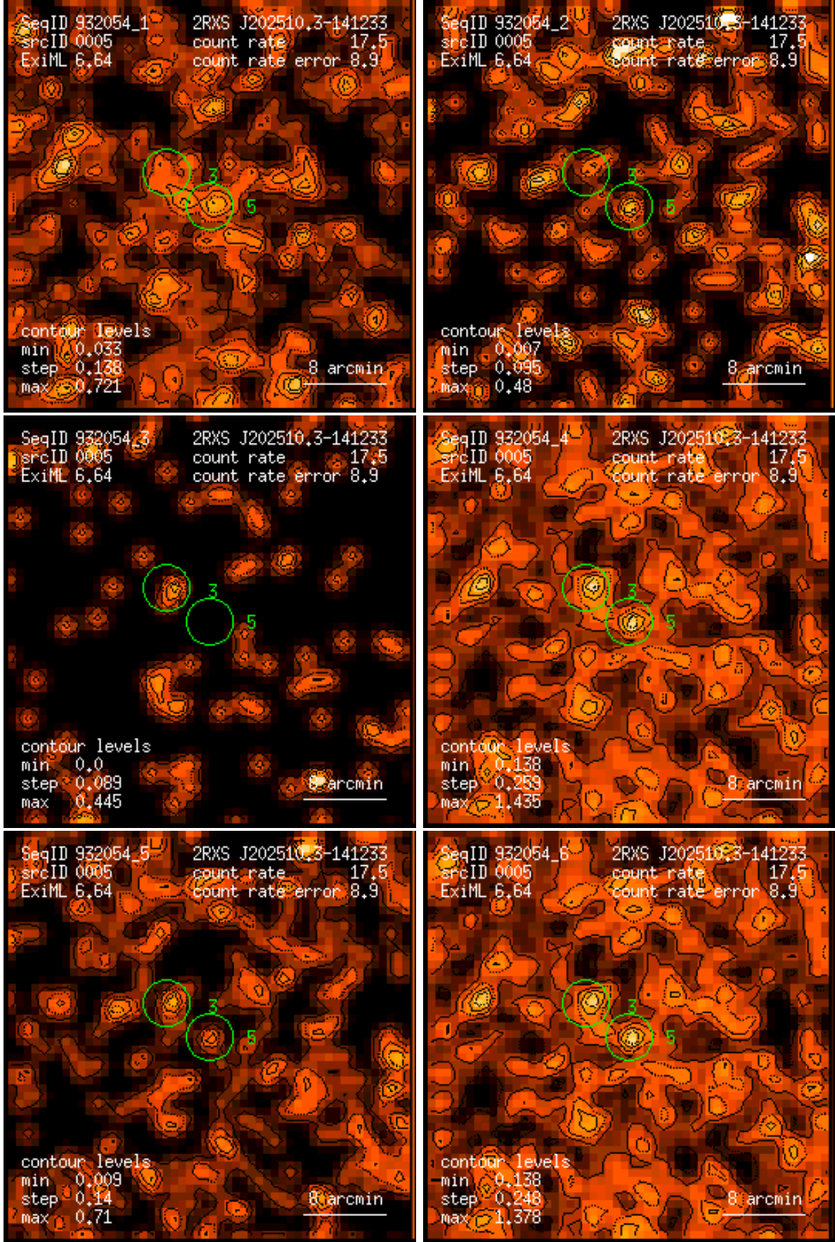
Figure 5: RASS 932054: detection 0005: band rate images, Gaussian filter: (1) PSPC channels 11 – 41, (2) 52 – 90, (3) 91 – 201, (4) 11 – 235, (5) 52 – 201, (6) 11 – 201. Broad band rates in counts/ks. Band rate contour levels in counts/ks/arcmin 2 .
