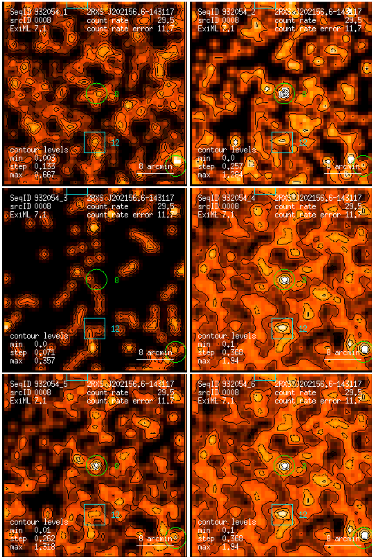
Figure 8: RASS 932054: detection 0008: band rate images, Gaussian filter: (1) PSPC channels 11 – 41, (2) 52 – 90, (3) 91 – 201, (4) 11 – 235, (5) 52 – 201, (6) 11 – 201. Broad band rates in counts/ks. Band rate contour levels in counts/ks/arcmin 2 .
