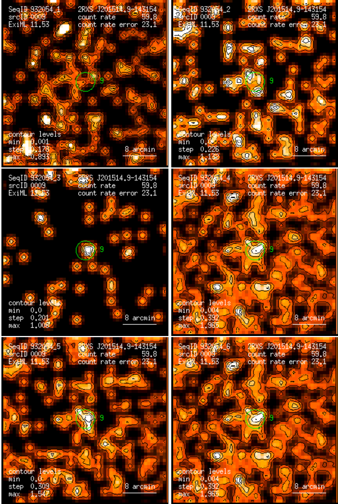
Figure 9: RASS 932054: detection 0009: band rate images, Gaussian filter: (1) PSPC channels 11 – 41, (2) 52 – 90, (3) 91 – 201, (4) 11 – 235, (5) 52 – 201, (6) 11 – 201. Broad band rates in counts/ks. Band rate contour levels in counts/ks/arcmin 2 .
