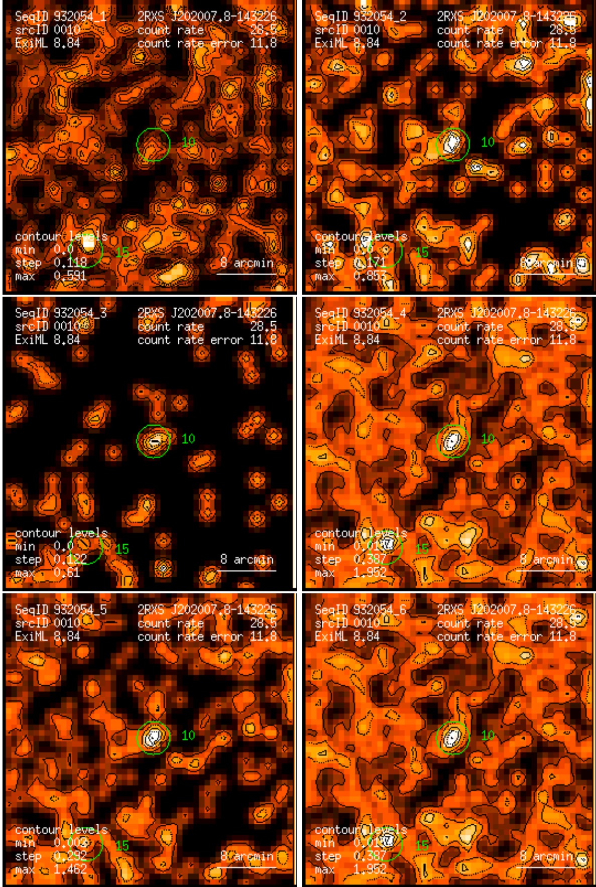
Figure 10: RASS 932054: detection 0010: band rate images, Gaussian filter: (1) PSPC channels 11 – 41, (2) 52 – 90, (3) 91 – 201, (4) 11 – 235, (5) 52 – 201, (6) 11 – 201. Broad band rates in counts/ks. Band rate contour levels in counts/ks/arcmin 2 .
